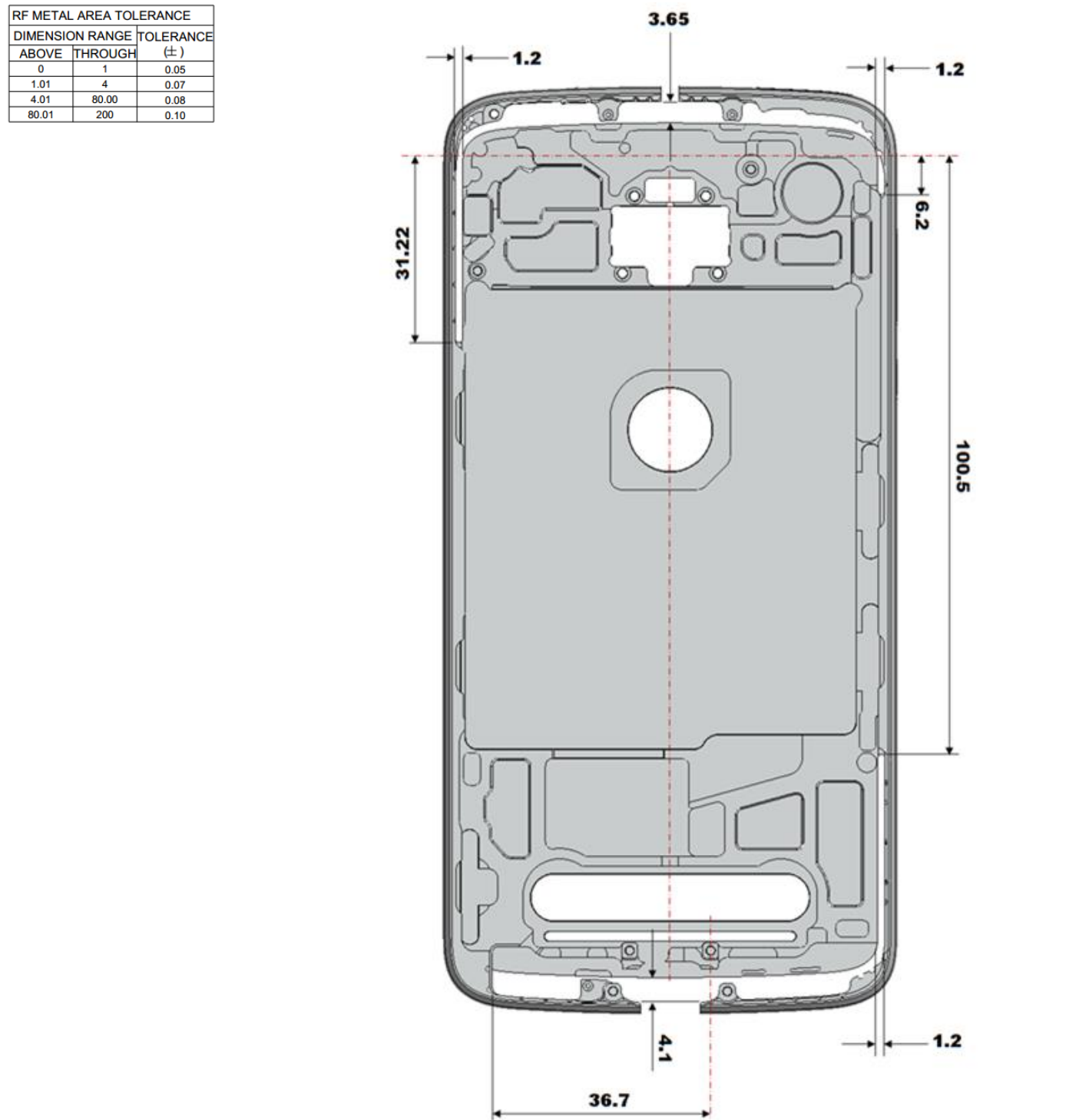
Photograph 9-8: Antenna Locations and Spacings.
