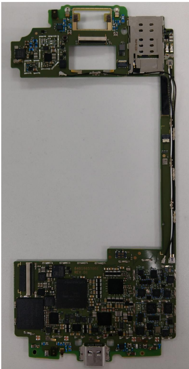
Photograph 9-3: PCB without Shields – Front (Display) Side
