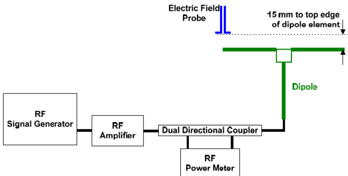
Fig. 7.1 Setup Diagram
