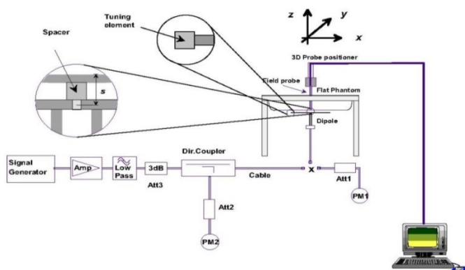
Fig 11.3.1 System Performance Check Setup
