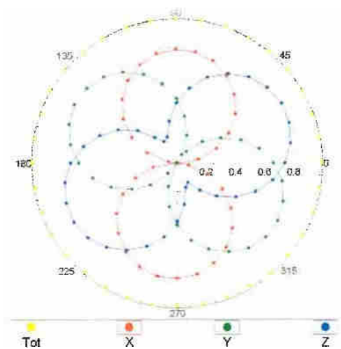
f=600 MHz,TEM
