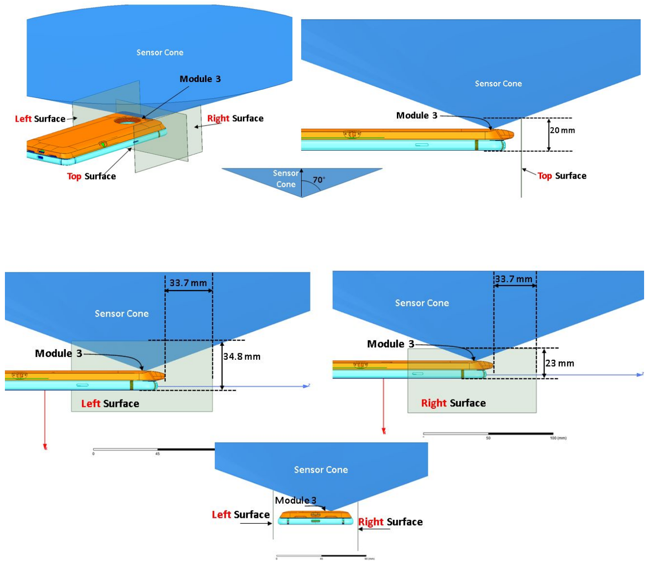
Figure 5.2.4.4 Measurement planes for Module 3.
