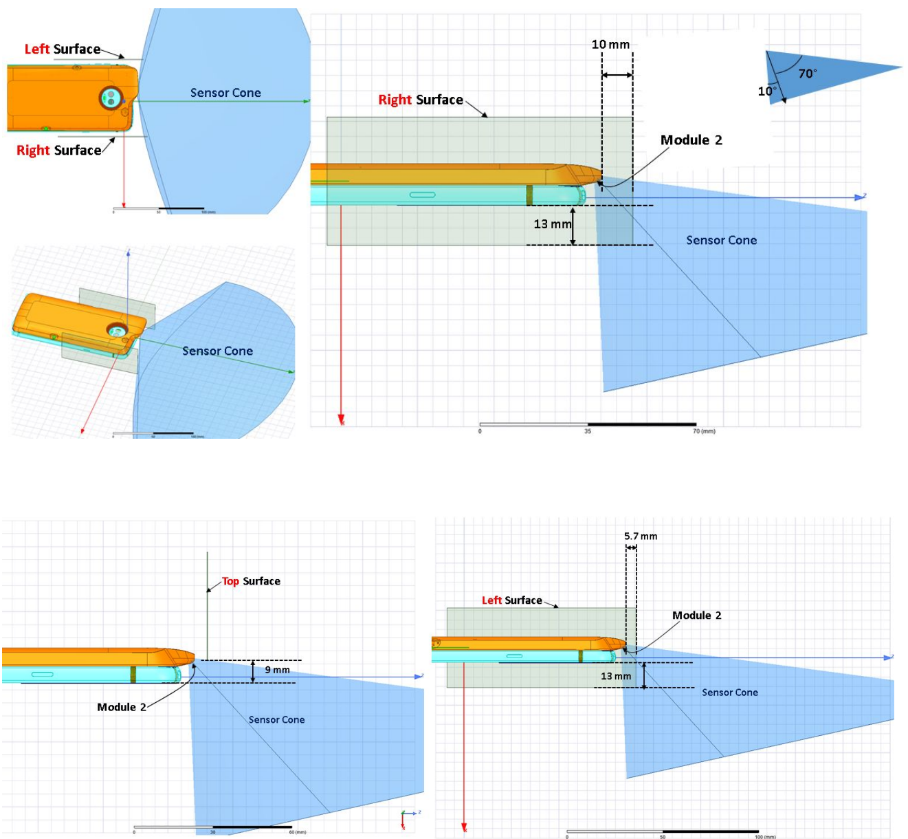
Figure 5.2.4.3 Measurement planes for Module 2.
