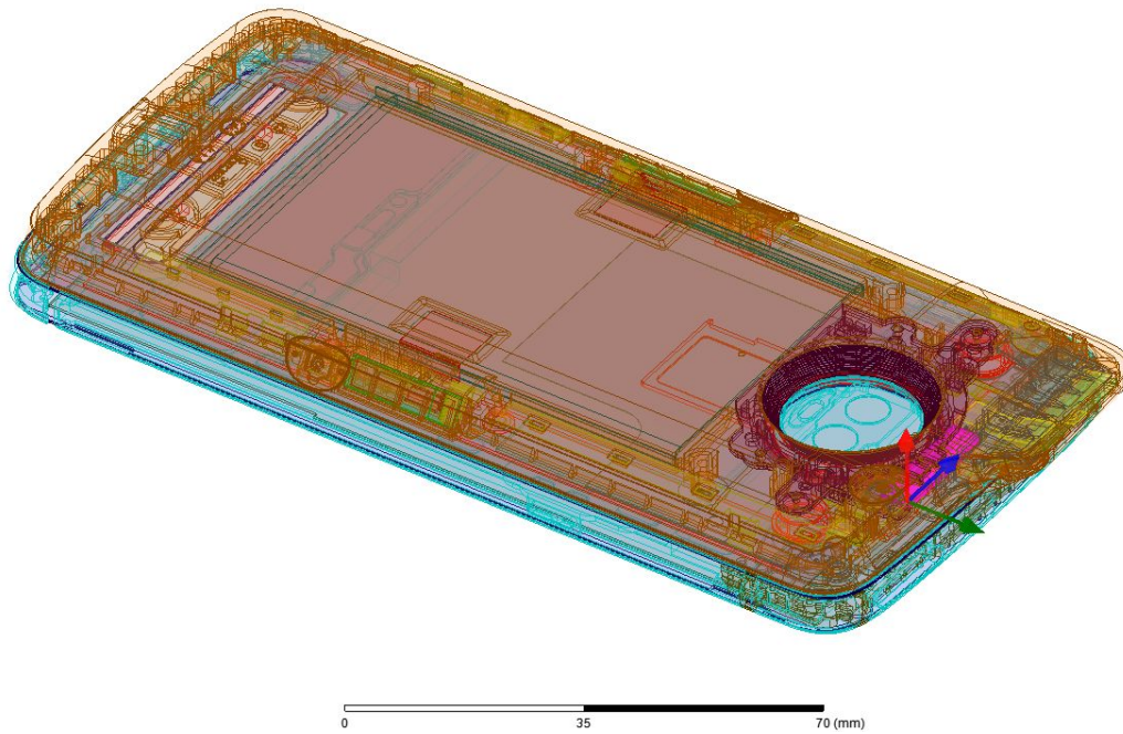
Figure 3.3.4-4: 3D model used for Module 3 (Back Array), the antenna array is highlighted
