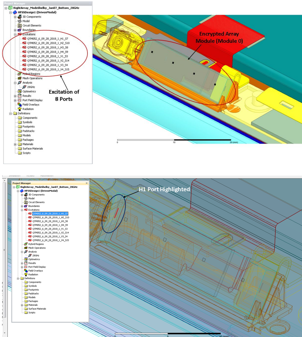
Figure 7.1.1-1: All 8 ports and the highlighted H1 port (Horizontal) in HFSS.
