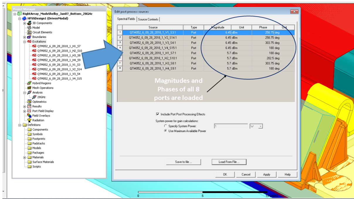
Figure 7.1.1-2: Magnitudes and phases of a beam pair are loaded in HFSS.
