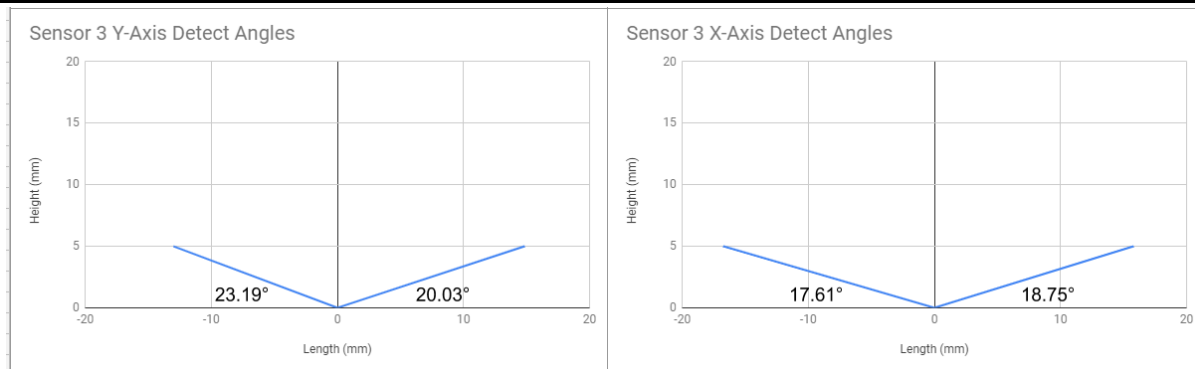
Measured angular responses of Sensor 3 at the 5 mm test separation distance.
