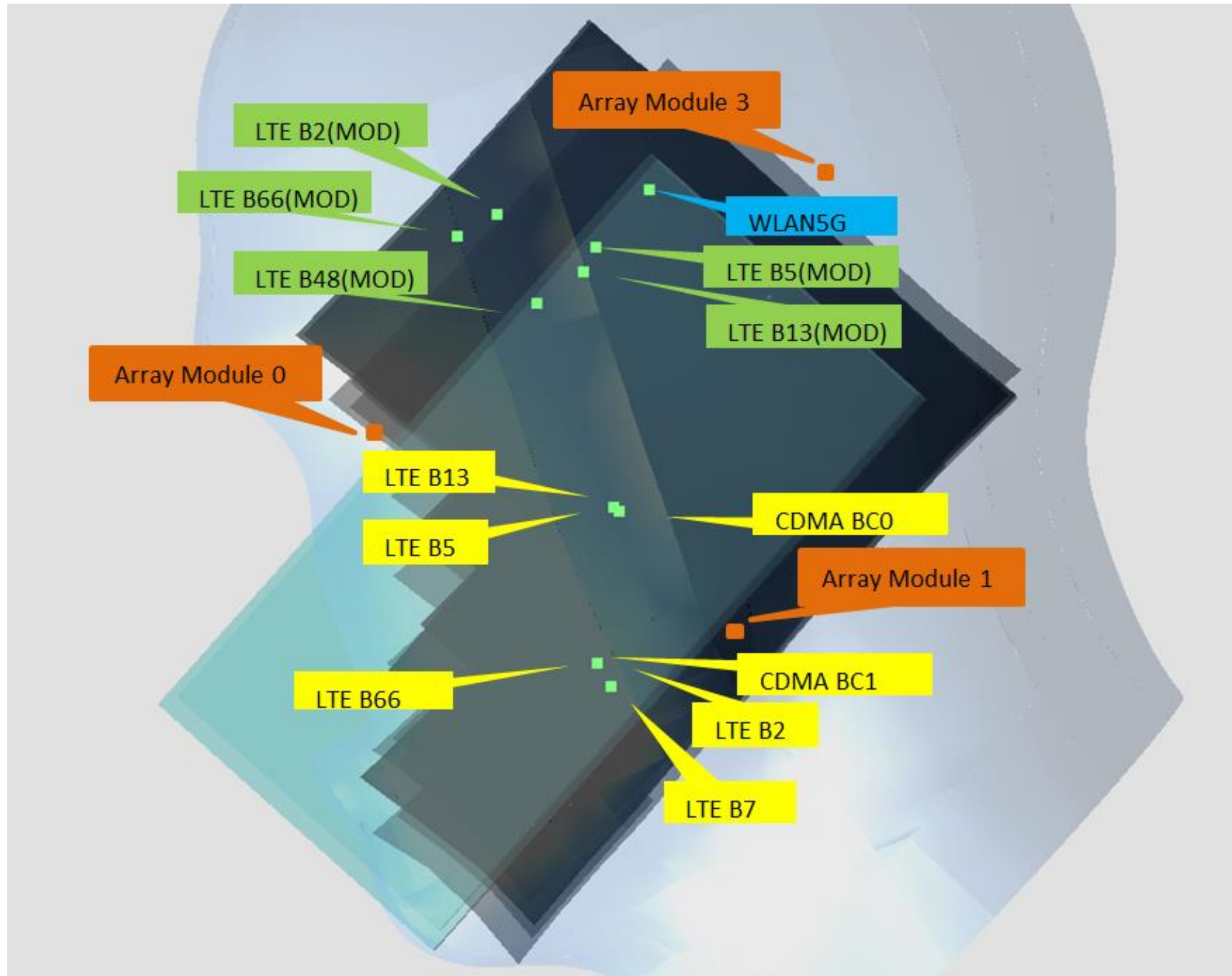
Each transmitter SAR and PD peak location for Right Cheek exposure position
