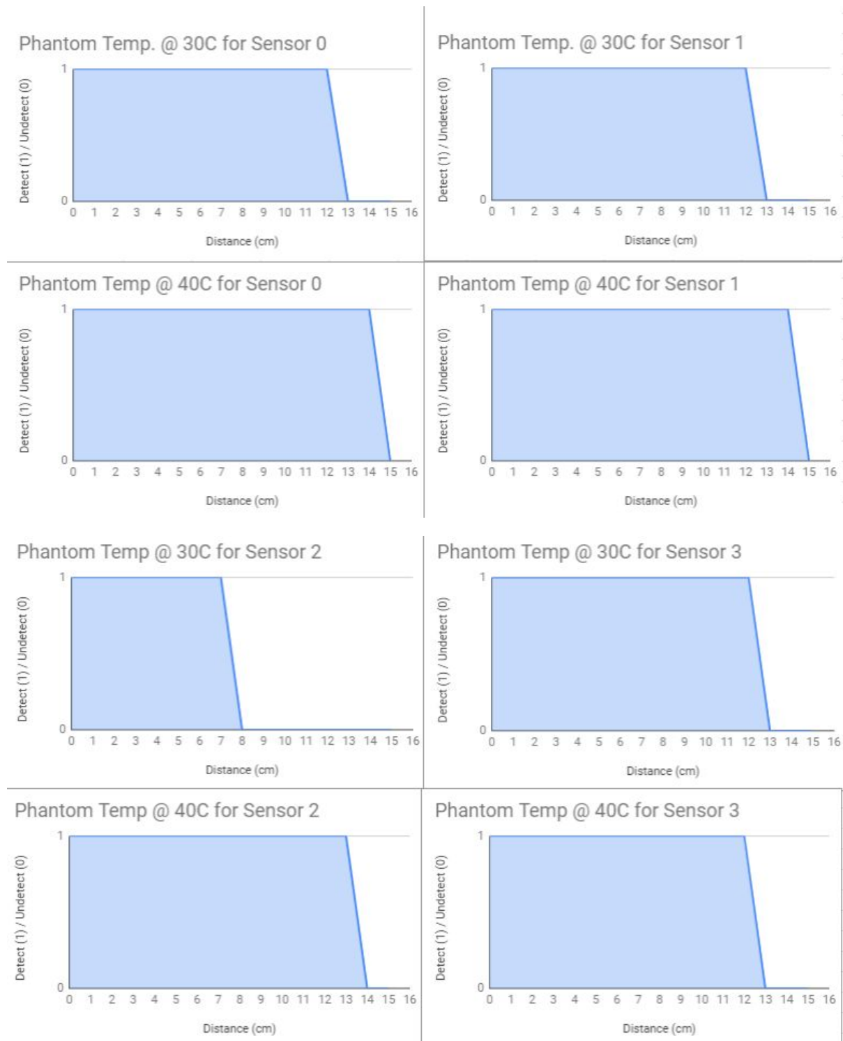
Figure 5.1-1: Trigger/Release distance test results.
