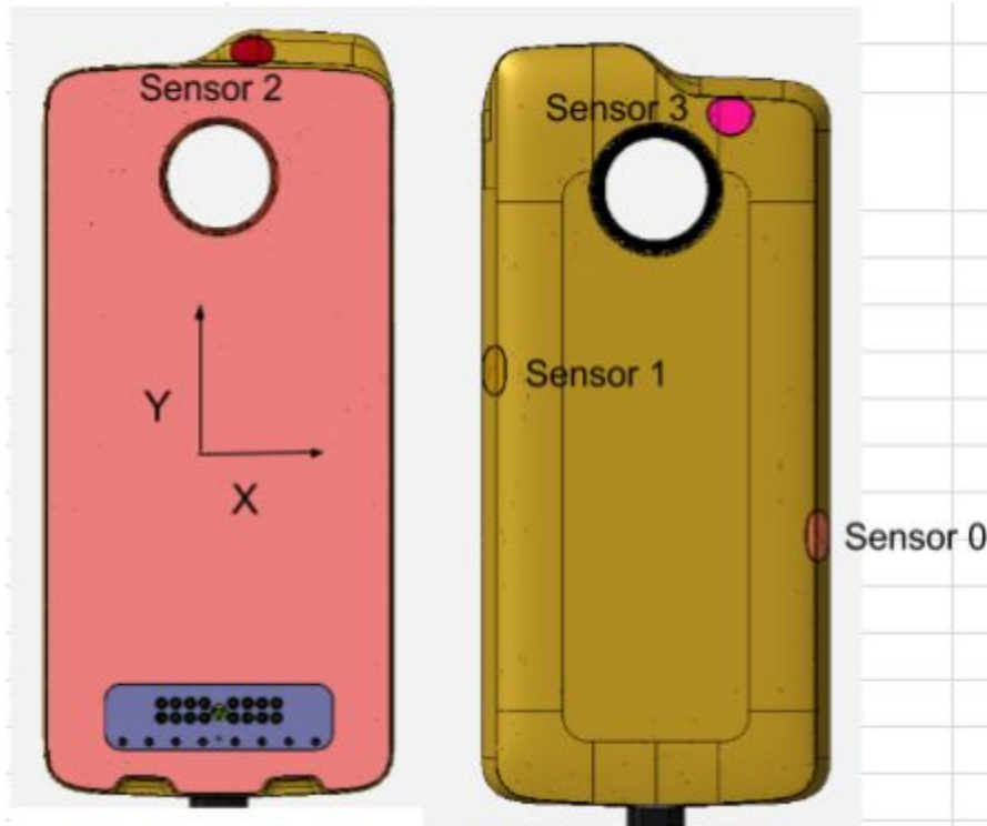
Figure 5-1: Reference numbers for sensors and the coordinate system.
