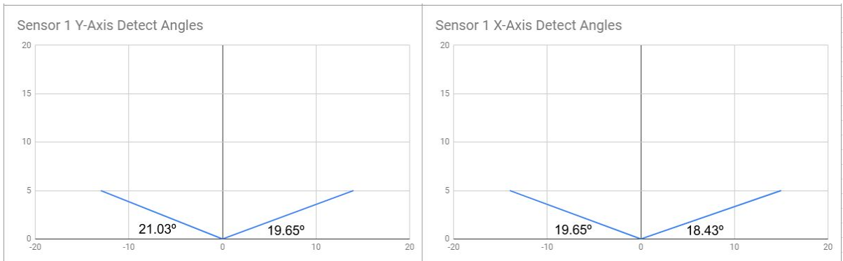
Figure 5.2-1(b): Measured angular responses of Sensor 1 at the 5 mm test separation distance.
