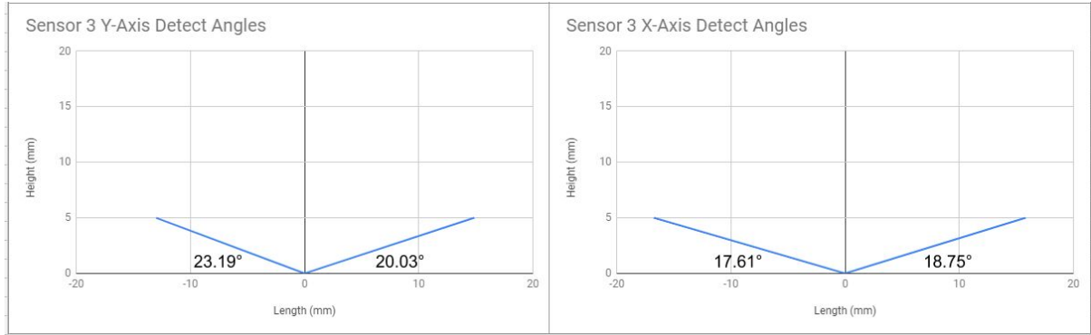
Figure 5.2-1(d): Measured angular responses of Sensor 3 at the 5 mm test separation distance.
