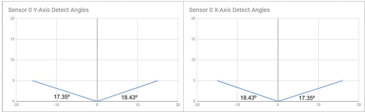
Figure 5.2-1(a): Measured angular responses of Sensor 0 at the 5 mm test separation distance.
