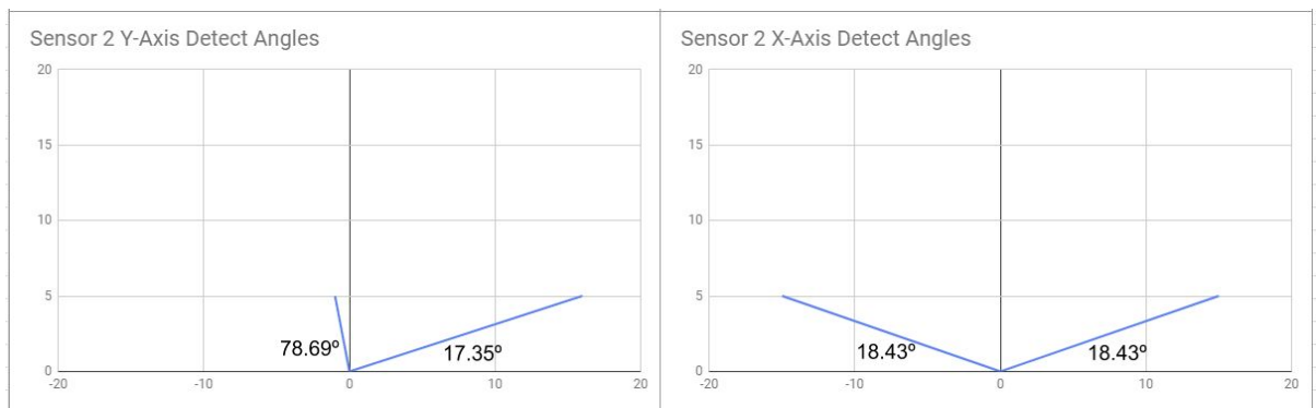
Figure 5.2-1(c): Measured angular responses of Sensor 2 at the 5 mm test separation distance.
