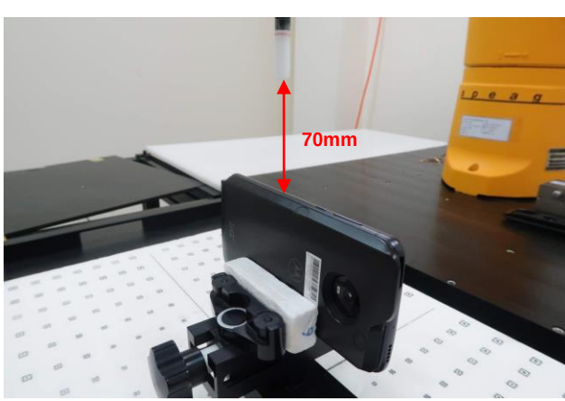
Left Side, Probe sensor to EUT surface distance 70mm
