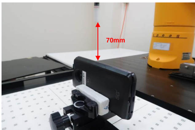
Right Side, Probe sensor to EUT surface distance 70mm
