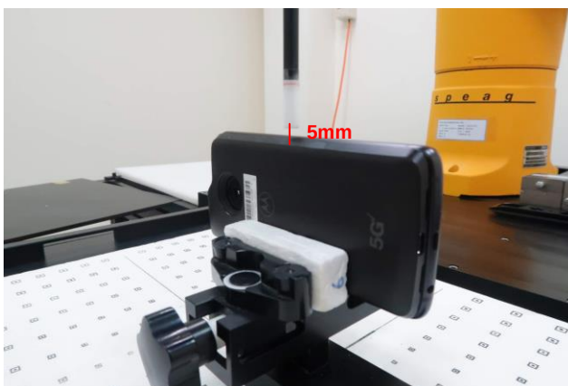
Right Side, Probe sensor to EUT surface distance 5mm
