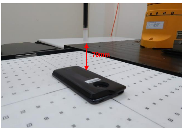
Back, Probe sensor to EUT surface distance 70mm
