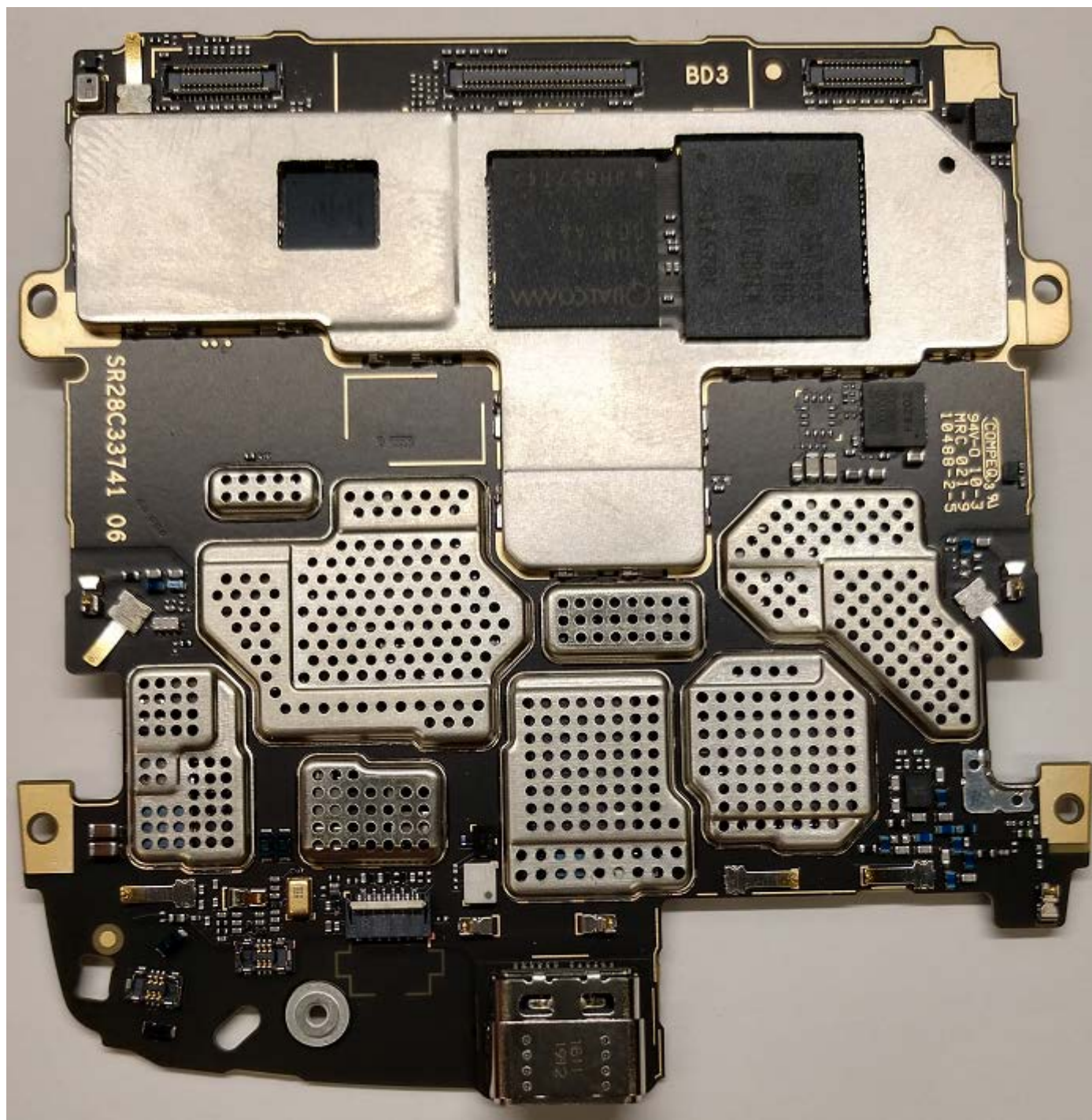
Photograph 9-1: PCB with Shields – Front (Display) Side
