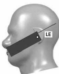
Fig 12.2.2 Handset vertical and horizontal reference lines—"clam-shell case"
