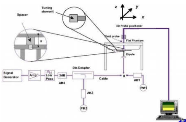
Fig 8.3.1 System Performance Check Setup
