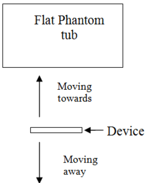
Sensor detection test set-up, front face
