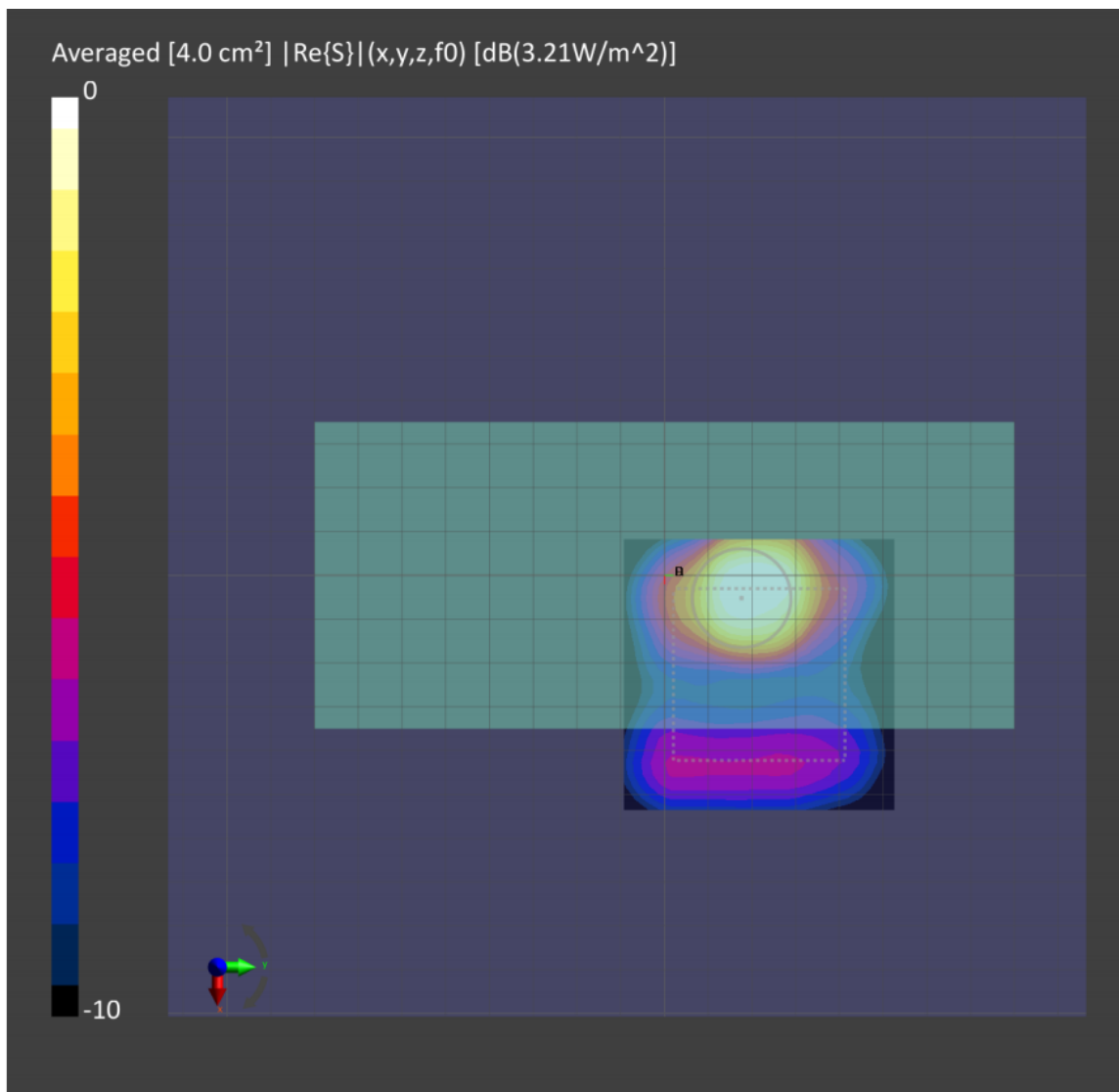
Figure 8-2: 4cm2-averaged power density distribution measured at input.power.limit of 3.7 dBm on the back surface for n261 beam 19
