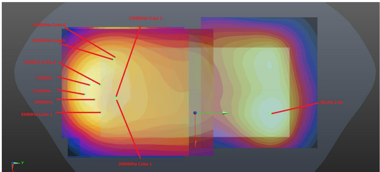
Front(5mm)+2.4G(5mm)
