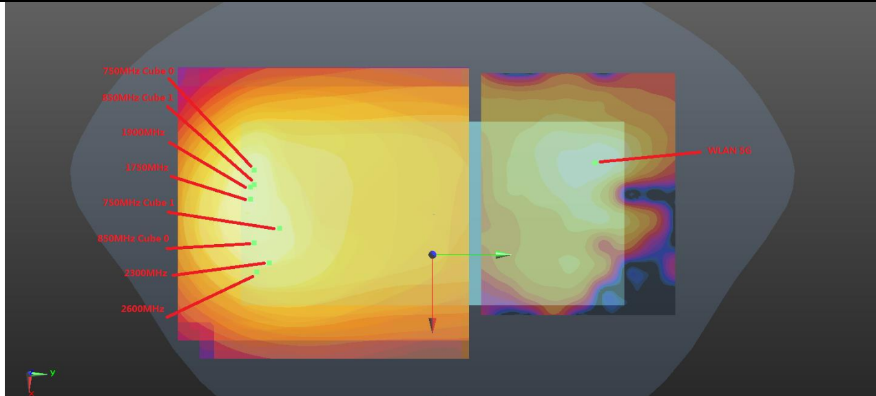
Back(5mm)+5G(5mm)
