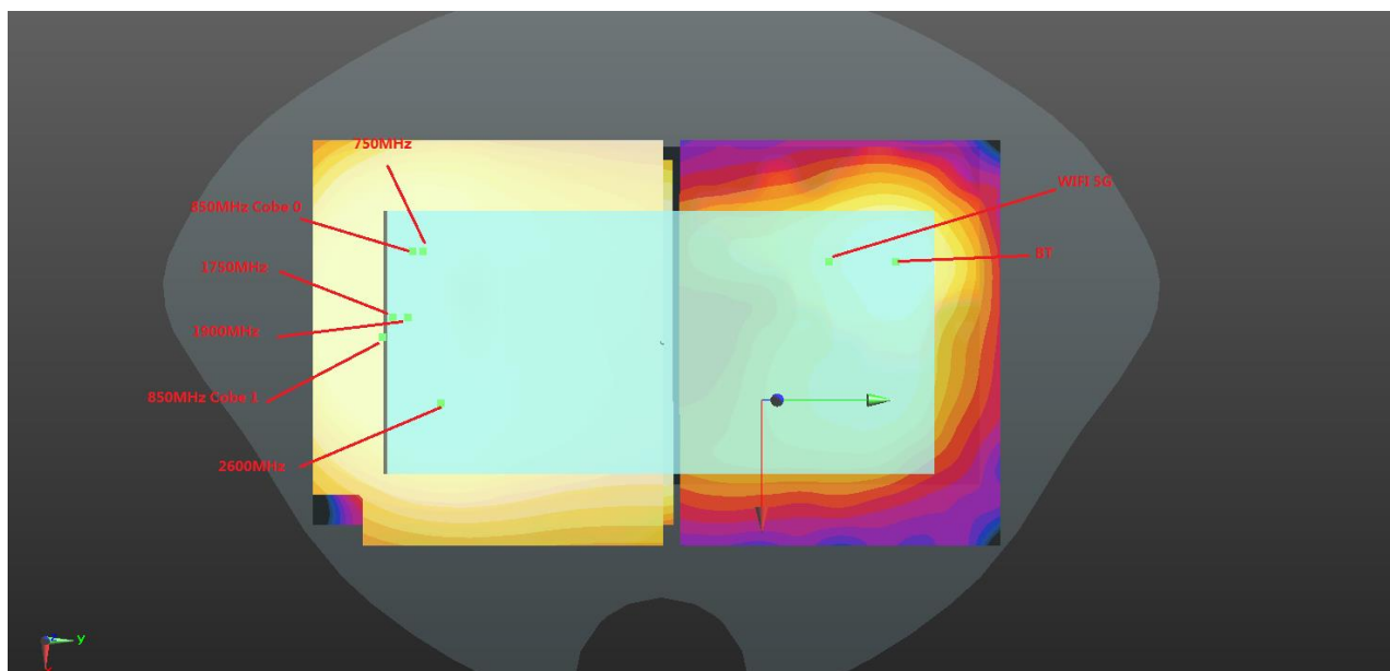
Back(5mm)+5G(5mm)+BT(5mm)
