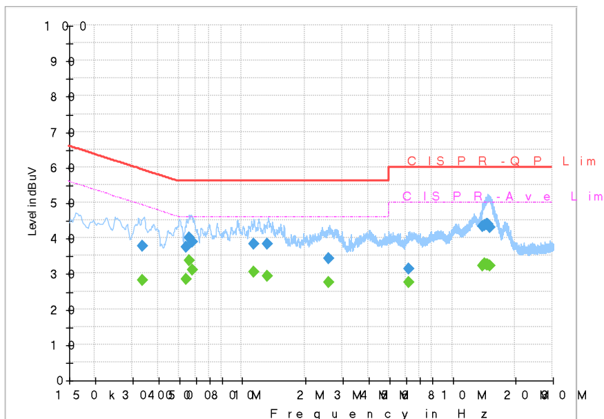
Full Spectrum
