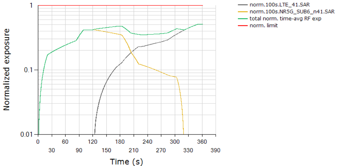
Total Normalized Time-averaged RF Exposure Tech: LTE, Band 41 / Tech: NR5G SUB6, Band n41
