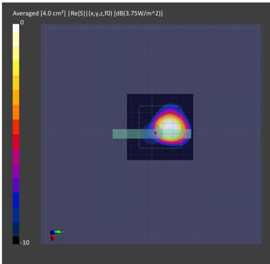
Figure 8-3: 4cm2-averaged power density distribution measured at input.power.limit of 4.44 dBm on the Back for n261 beam 15
