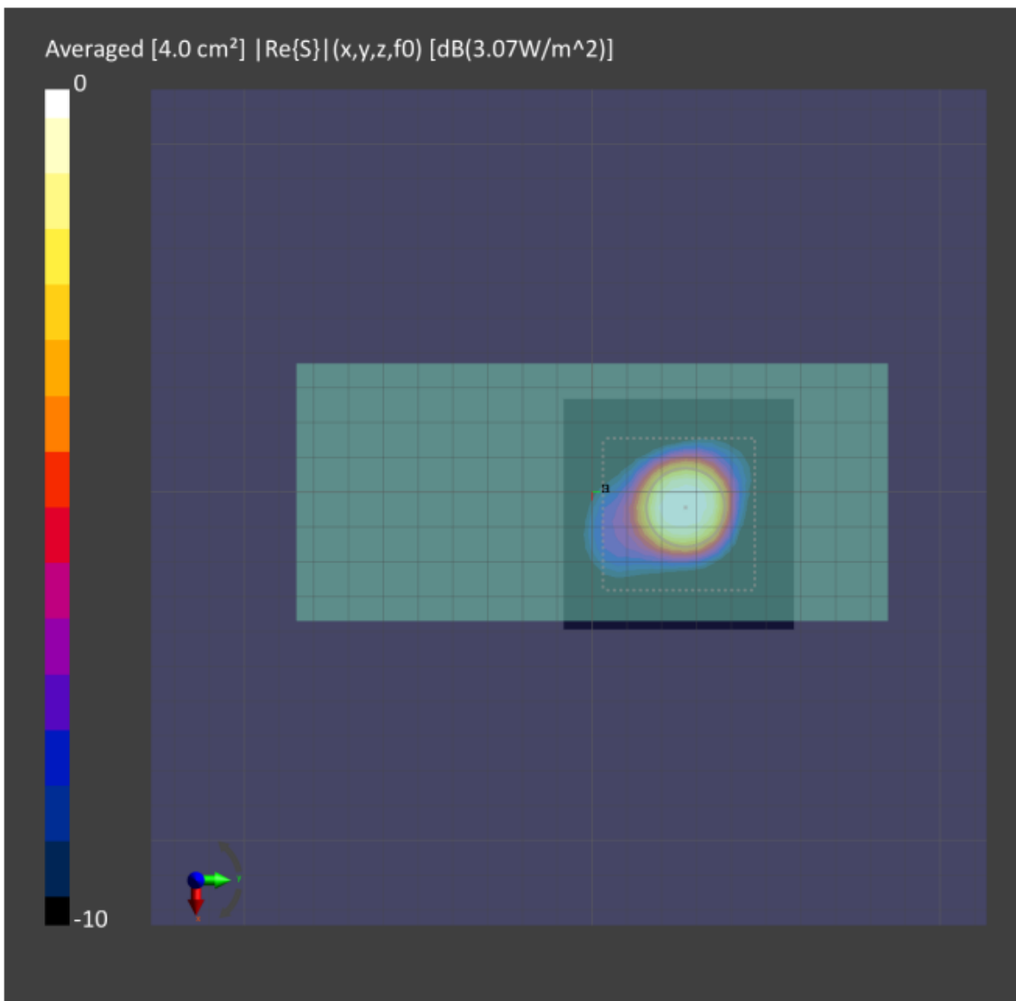
Figure 8-2: 4cm 2 -averaged power density distribution measured at input.power.limit of 8.5dBm on the back surface for n260 beam 1
