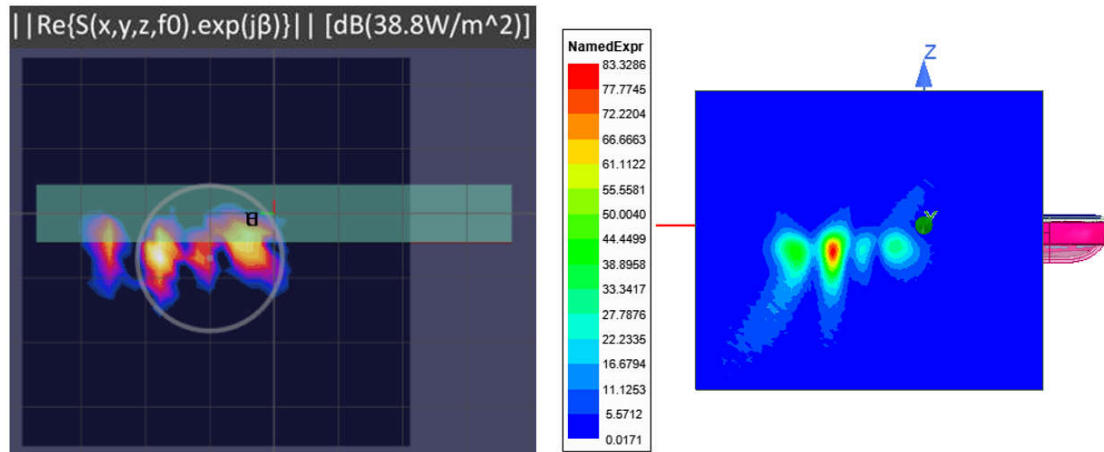
Figure 2.3.7.1-23 Measured (left) and Simulated (right) peak power density distributions for the worst case found in the Top surface measurement plane for n260 ( Top module, beam 15, top surface )
