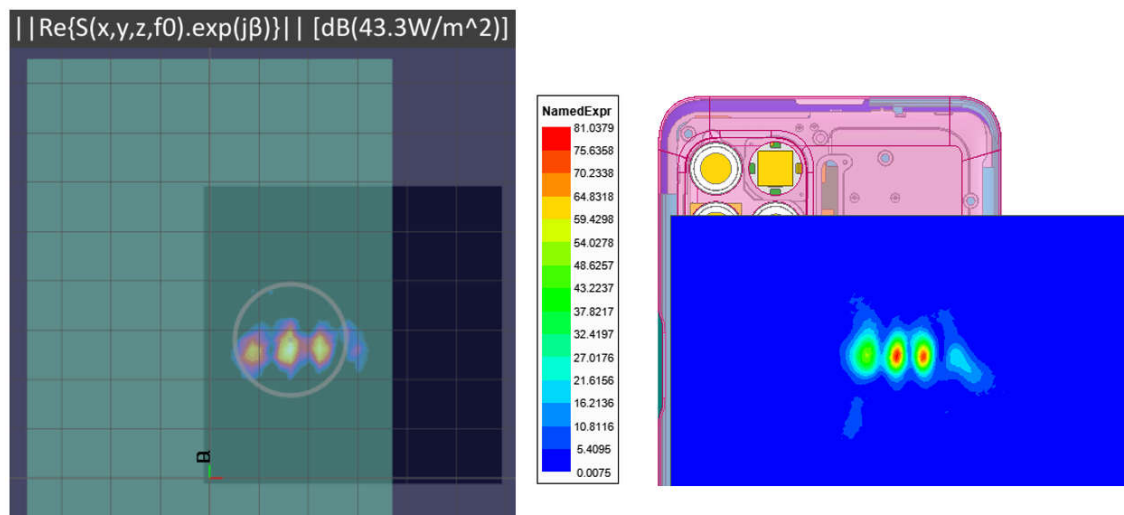
Figure 2.3.7.1-20 Measured (left) and Simulated (right) peak power density distributions for the worst case found in the Top surface measurement plane for n260 ( Back module, beam 148, back surface )
