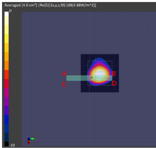
Figure 2.3.7.1-6 Measured (left) and Simulated (right) peak power density distributions for the worst case found in the Top surface measurement plane for n261 ( Top module, beam 152, top surface )
