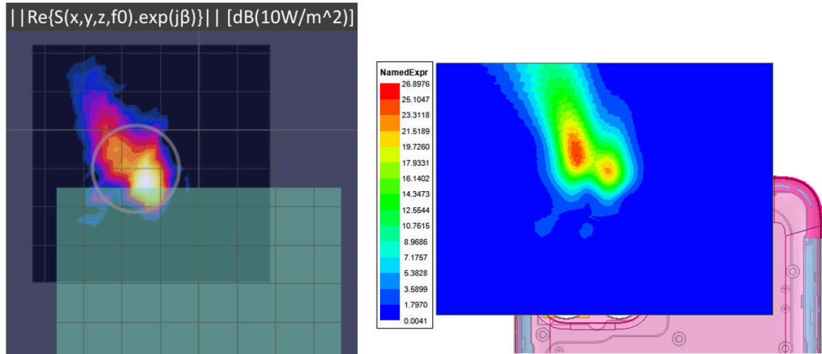
Figure 2.3.7.1-15 Measured (left) and Simulated (right) peak power density distributions for the worst case found in the Top surface measurement plane for n261 ( Top module, beam 15, back surface )
