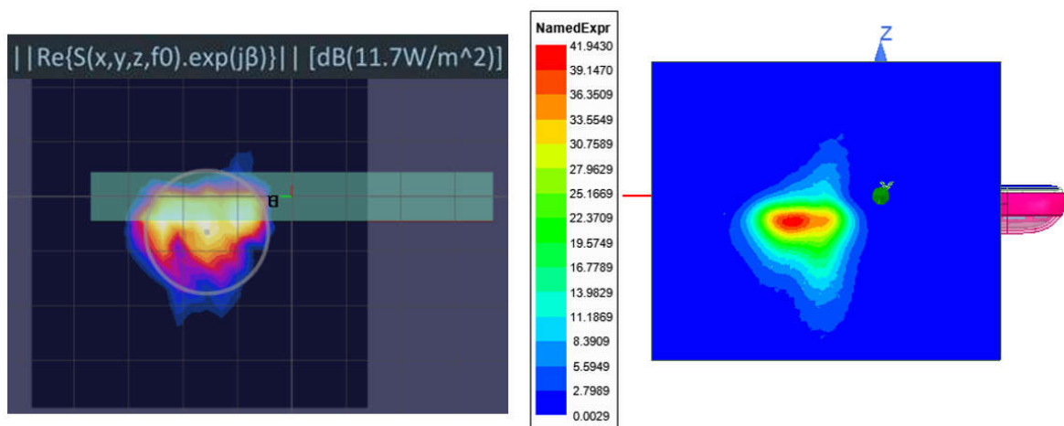
Figure 2.3.7.1-18 Measured (left) and Simulated (right) peak power density distributions for the worst case found in the Top surface measurement plane for n261 ( Top module, beam 152, top surface )
