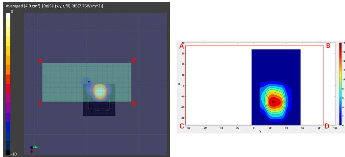
Figure 2.3.7.1-2 Measured (left) and Simulated (right) peak power density distributions for the worst case found in the back surface measurement plane for n261 ( Back module, beam 156, back surface )
