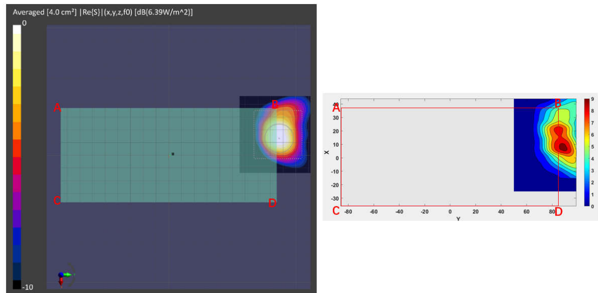
Figure 2.3.7.1-10 Measured (left) and Simulated (right) peak power density distributions for the worst case found in the Top surface measurement plane for n260 ( Top module, beam 153, back surface )
