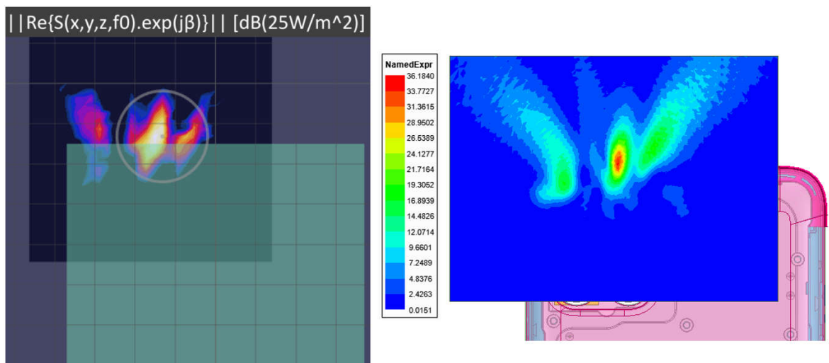
Figure 2.3.7.1-22 Measured (left) and Simulated (right) peak power density distributions for the worst case found in the Top surface measurement plane for n260 ( Top module, beam 153, back surface )
