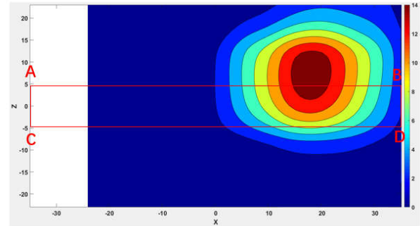
Figure 2.3.7.1-5 Measured (left) and Simulated (right) peak power density distributions for the worst case found in the Top surface measurement plane for n261 ( Top module, beam 15, top surface )
