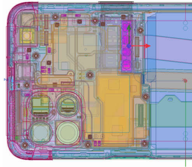
Figure 2.3.4-1: 3D model used for Module 0 (Back module), the antenna array is highlighted
