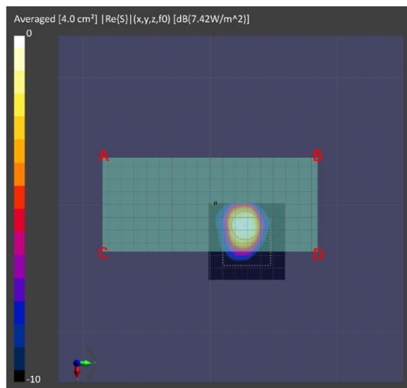
Figure 2.3.7.1-8 Measured (left) and Simulated (right) peak power density distributions for the worst case found in the back surface measurement plane for n260 ( Back module, beam 148, back surface )
