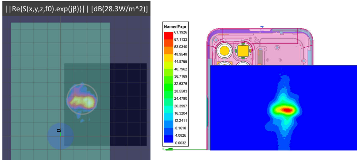
Figure 2.3.7.1-13 Measured (left) and Simulated (right) peak power density distributions for the worst case found in the Top surface measurement plane for n261 ( Back module, beam 19, back surface )
