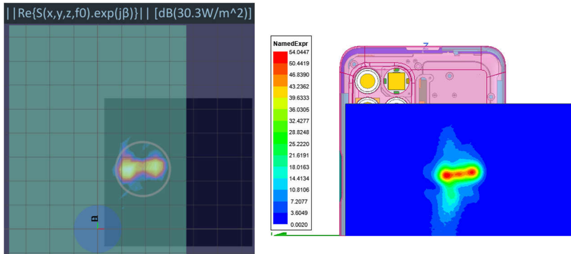
Figure 2.3.7.1-14 Measured (left) and Simulated (right) peak power density distributions for the worst case found in the Top surface measurement plane for n261 ( Back module, beam 156, back surface )
