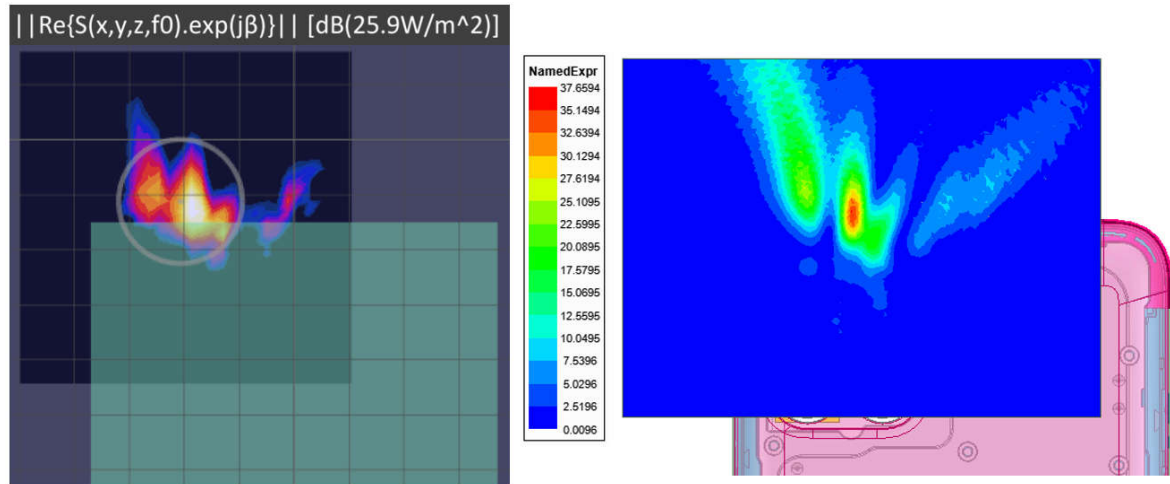
Figure 2.3.7.1-21 Measured (left) and Simulated (right) peak power density distributions for the worst case found in the Top surface measurement plane for n260 ( Top module, beam 24, back surface )
