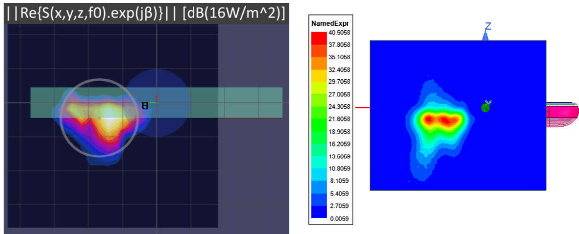
Figure 2.3.7.1-17 Measured (left) and Simulated (right) peak power density distributions for the worst case found in the Top surface measurement plane for n261 ( Top module, beam 15, top surface )
