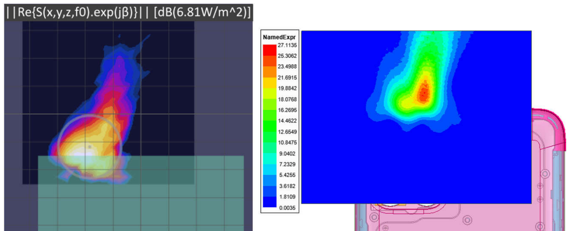
Figure 2.3.7.1-16 Measured (left) and Simulated (right) peak power density distributions for the worst case found in the Top surface measurement plane for n261 ( Top module, beam 152, back surface )
