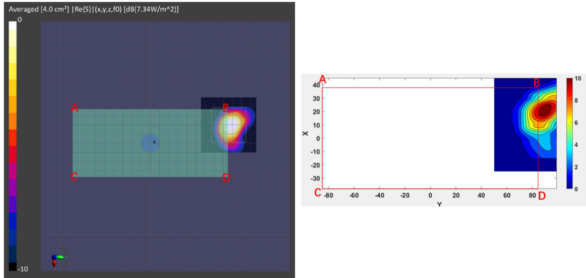
Figure 2.3.7.1-9 Measured (left) and Simulated (right) peak power density distributions for the worst case found in the Top surface measurement plane for n261 ( Top module, beam 24, back surface )
