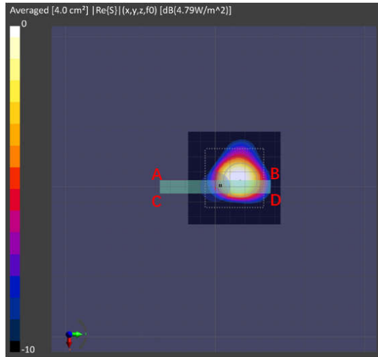
Figure 2.3.7.1-5 Measured (left) and Simulated (right) peak power density distributions for the worst case found in the Top surface measurement plane for n261 ( Top module, beam 15, top surface )
