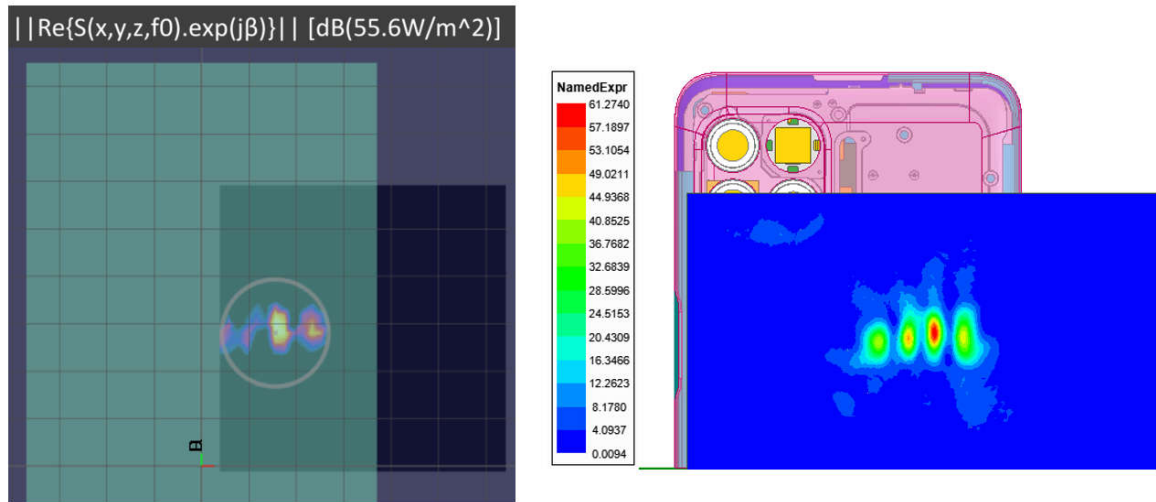
Figure 2.3.7.1-19 Measured (left) and Simulated (right) peak power density distributions for the worst case found in the Top surface measurement plane for n260 ( Back module, beam 29, back surface )
