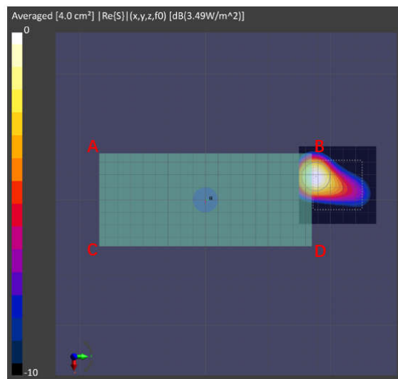
Figure 2.3.7.1-4 Measured (left) and Simulated (right) peak power density distributions for the worst case found in the Top surface measurement plane for n261 ( Top module, beam 152, back surface )
