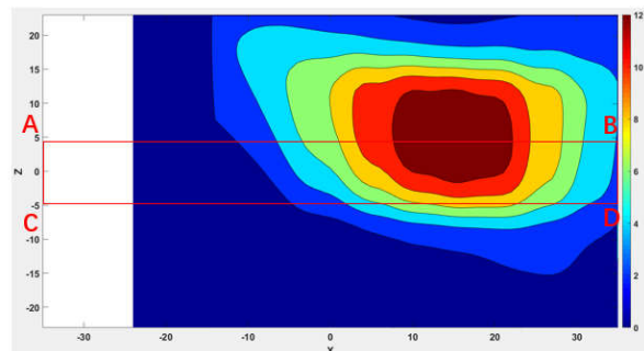
Figure 2.3.7.1-12 Measured (left) and Simulated (right) peak power density distributions for the worst case found in the Top surface measurement plane for n260 ( Top module, beam 144, top surface )
