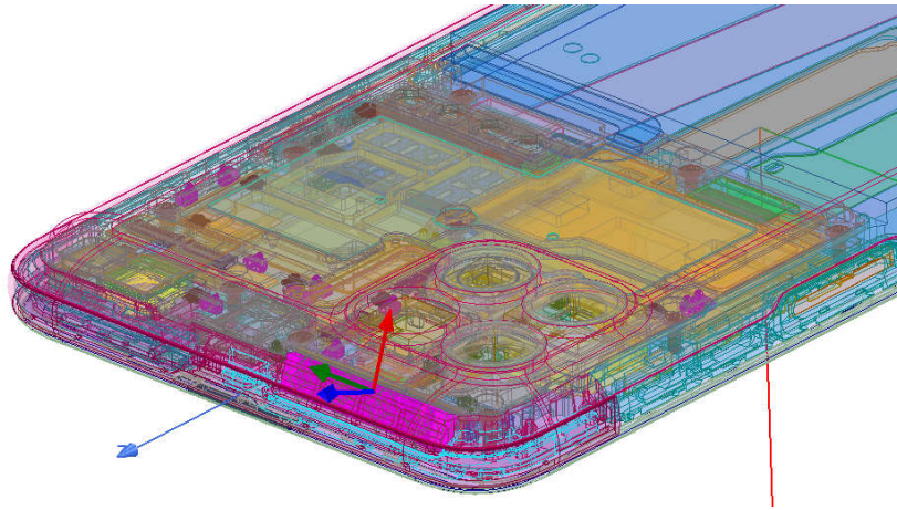
Figure 2.3.4-1: 3D model used for Module 1 (Top module), the antenna array is highlighted
