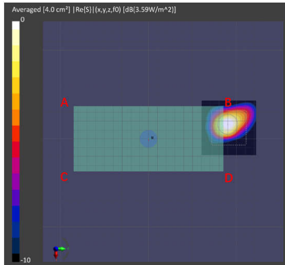
Figure 2.3.7.1-3 Measured (left) and Simulated (right) peak power density distributions for the worst case found in the Top surface measurement plane for n261 ( Top module, beam 15, back surface )
