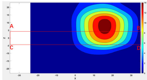
Figure 2.3.7.1-6 Measured (left) and Simulated (right) peak power density distributions for the worst case found in the Top surface measurement plane for n261 ( Top module, beam 152, top surface )
