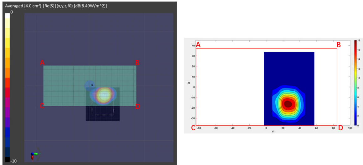
Figure 2.3.7.1-1 Measured (left) and Simulated (right) peak power density distributions for the worst case found in the back surface measurement plane for n261 ( Back module, beam 19, back surface )
