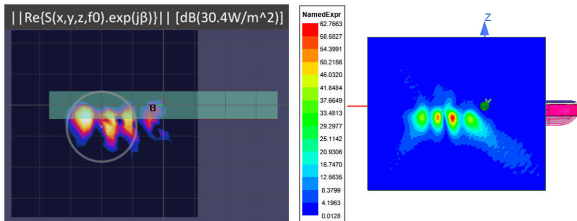
Figure 2.3.7.1-24 Measured (left) and Simulated (right) peak power density distributions for the worst case found in the Top surface measurement plane for n260 ( Top module, beam 144, top surface )
