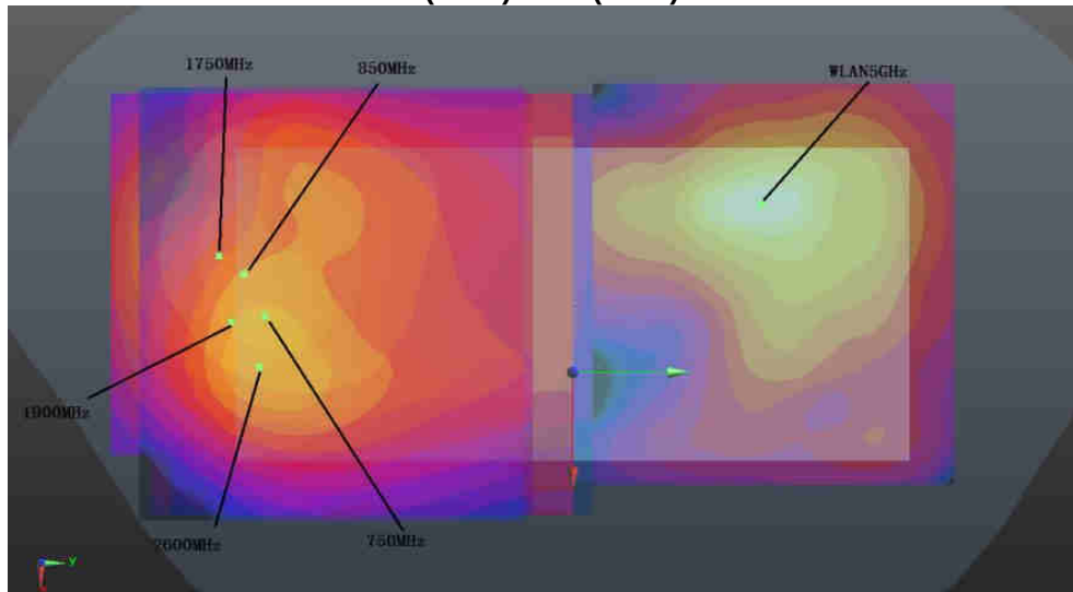
WWAN(5mm)+5G(5mm) Back
