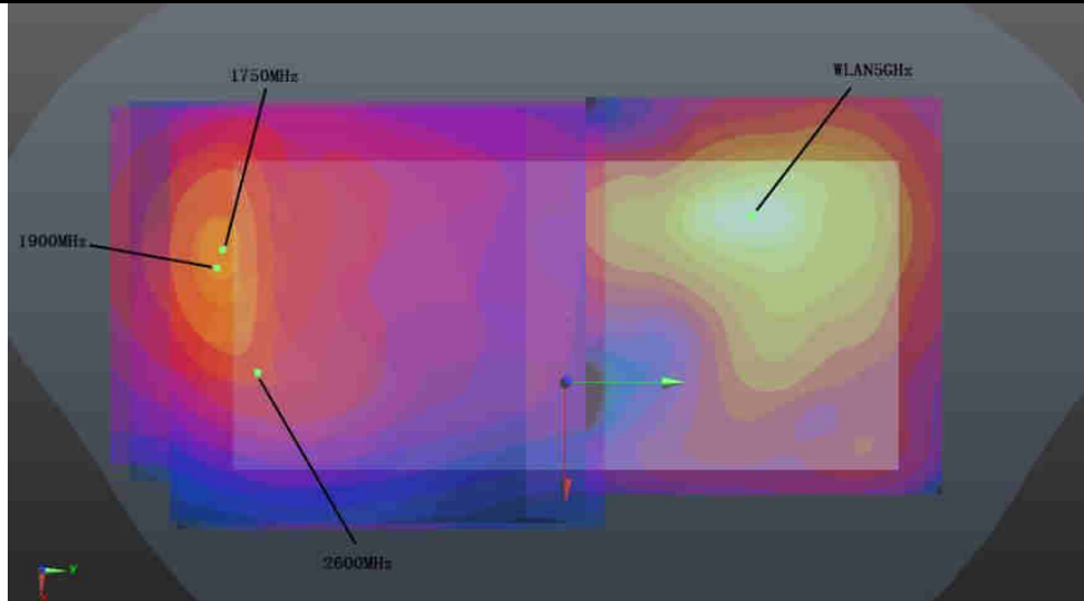
WWAN(0mm)+5G(0mm) Back
