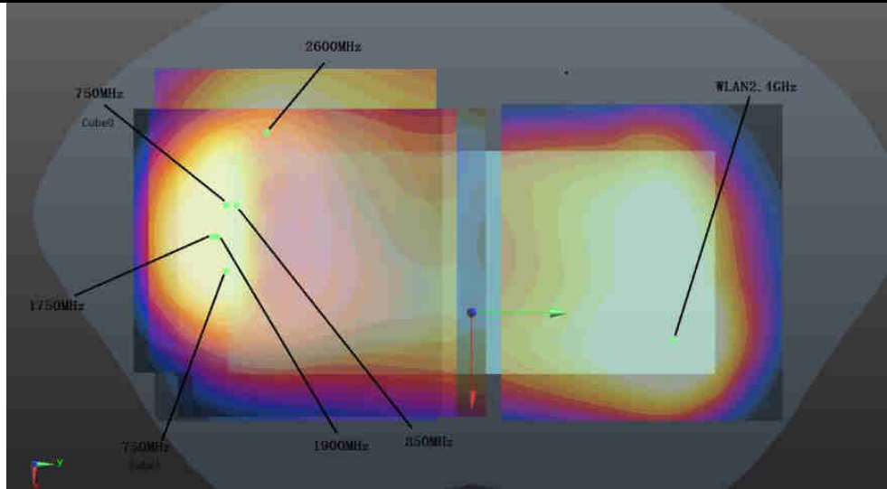
WWAN(5mm)+2.4G(5mm) Front
