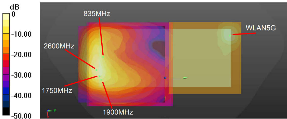
Back(0mm)+ WLAN5GHz(0mm)
