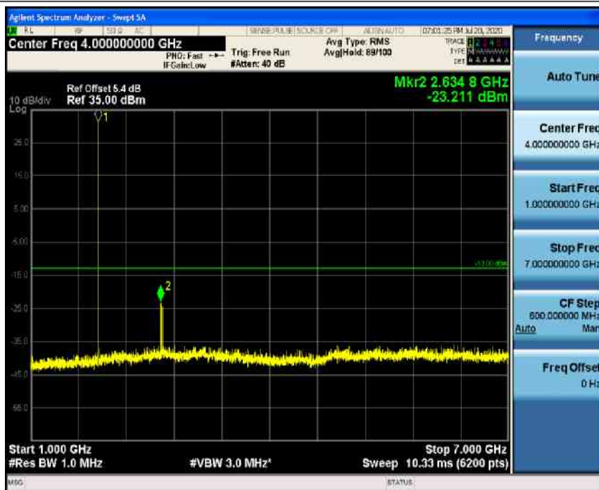
GSM1900_512
