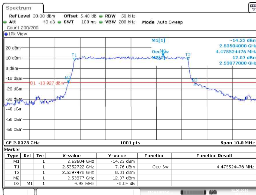
Band41-5MHz-QPSK-40065-25RB#0-4.476
