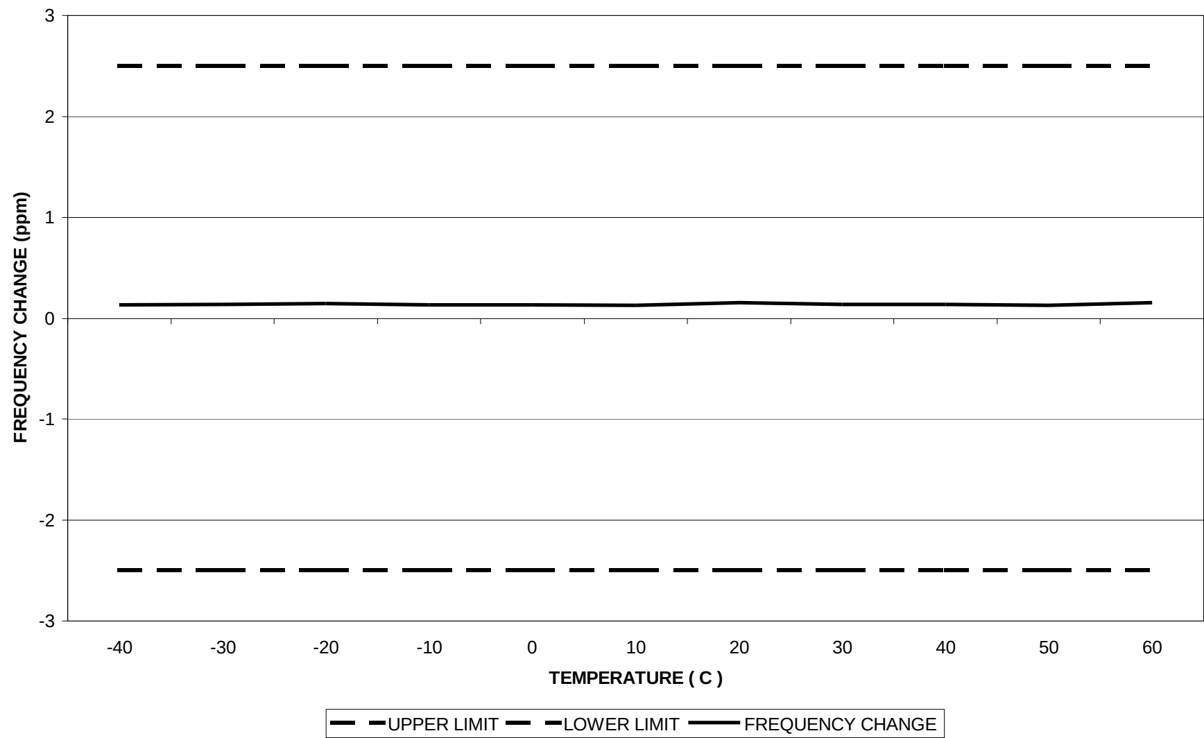
REFERENCE OSCILLATOR FREQUENCY STABILITY VS TEMPERATURE ANALOG MODE
