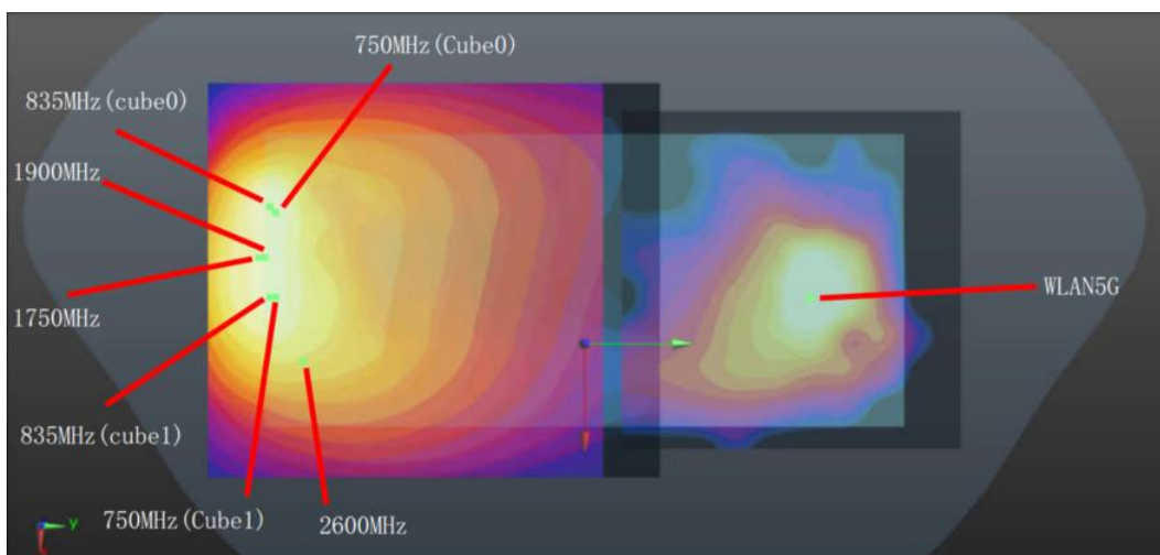
Back for WWAN+WLAN5GHz_0mm
