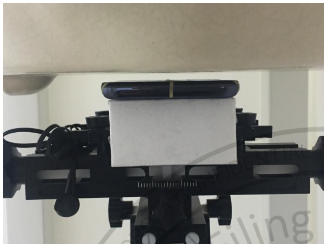
Front with handset, Test Separation 5 mm
