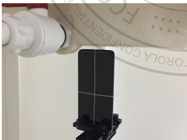
Bottom Side, Test Separation 6 mm
