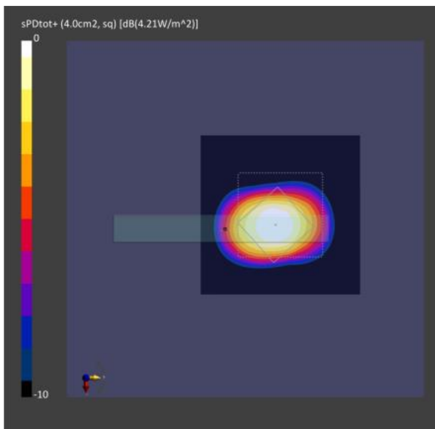
Figure 8-2: 4cm2-averaged power density distribution measured at input.power.limit of 4.21 dBm on the Right Side surface for n260 beam 15
