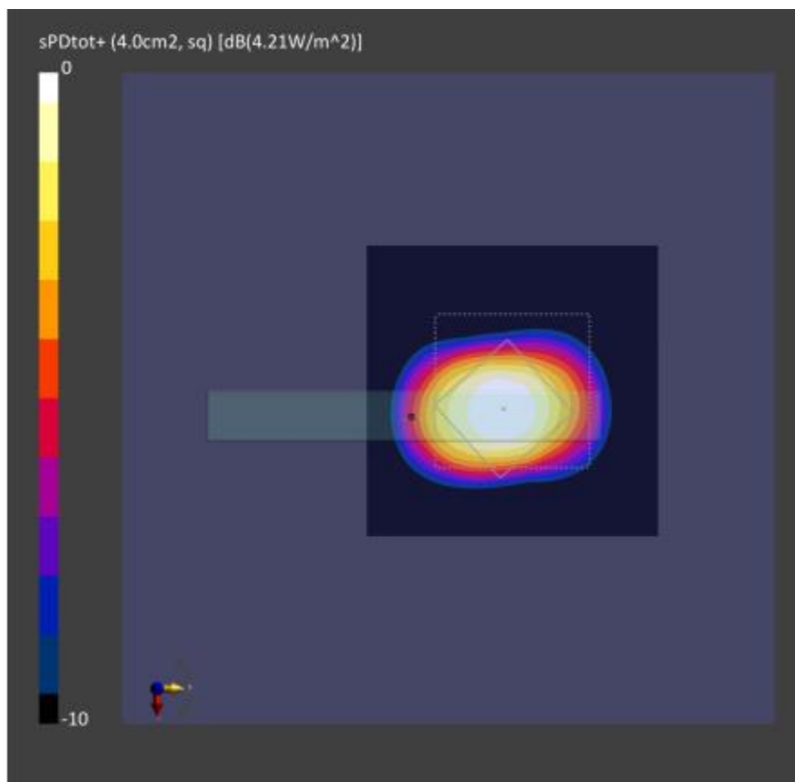
Figure 8-3: 4cm2-averaged power density distribution measured at input.power.limit of 4.21 dBm on the Right Side surface for n260 beam 15
