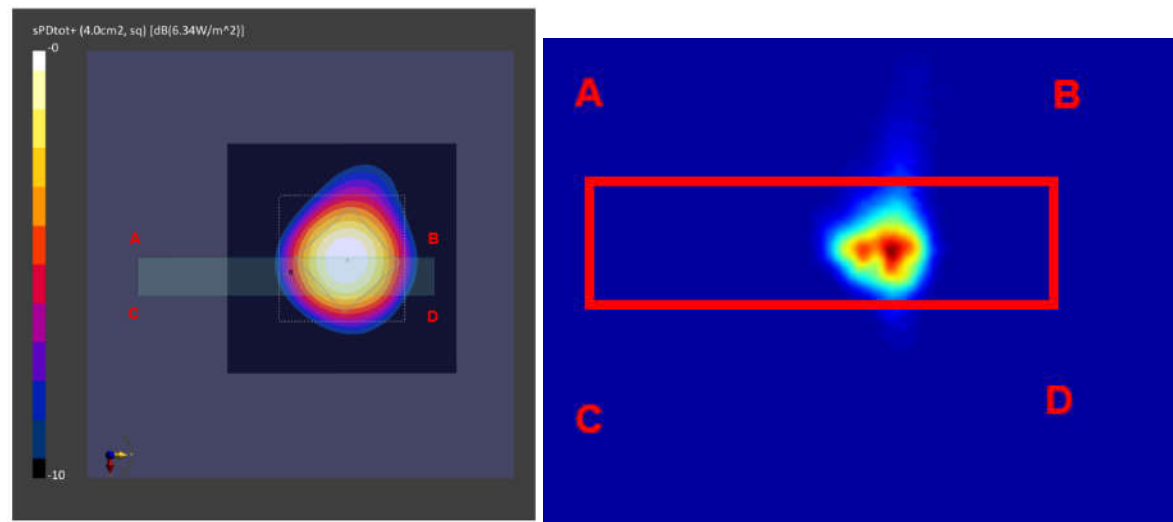
Figure 2.3.7.1-5 Measured (left) and Simulated (right) peak power density distributions for the worst case found in the Top surface measurement plane for n261 ( Top module, beam 23, top surface )
