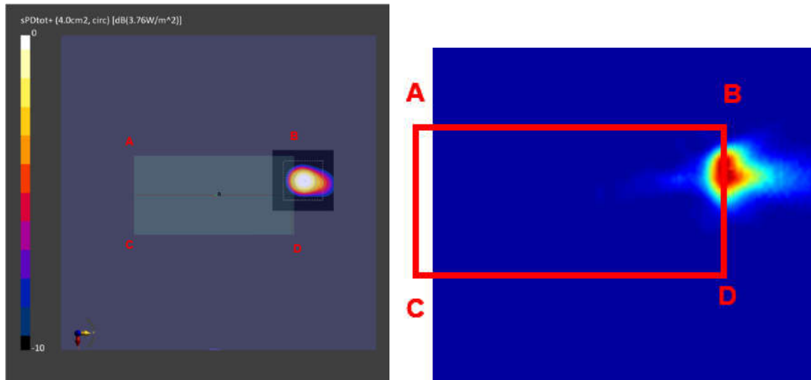
Figure 2.3.7.1-4 Measured (left) and Simulated (right) peak power density distributions for the worst case found in the Top surface measurement plane for n261 ( Top module, beam 142, back surface )
