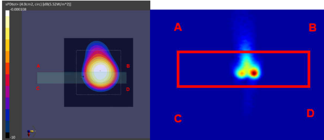
Figure 2.3.7.1-6 Measured (left) and Simulated (right) peak power density distributions for the worst case found in the Top surface measurement plane for n261 ( Top module, beam 142, top surface )
