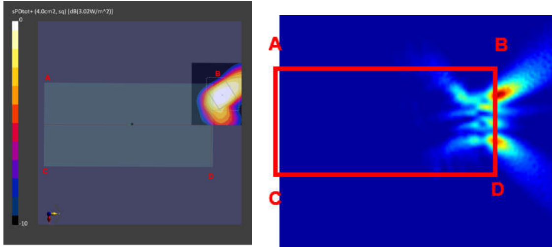
Figure 2.3.7.1-8 Measured (left) and Simulated (right) peak power density distributions for the worst case found in the back surface measurement plane for n260 ( Back module, beam 15, back surface )
