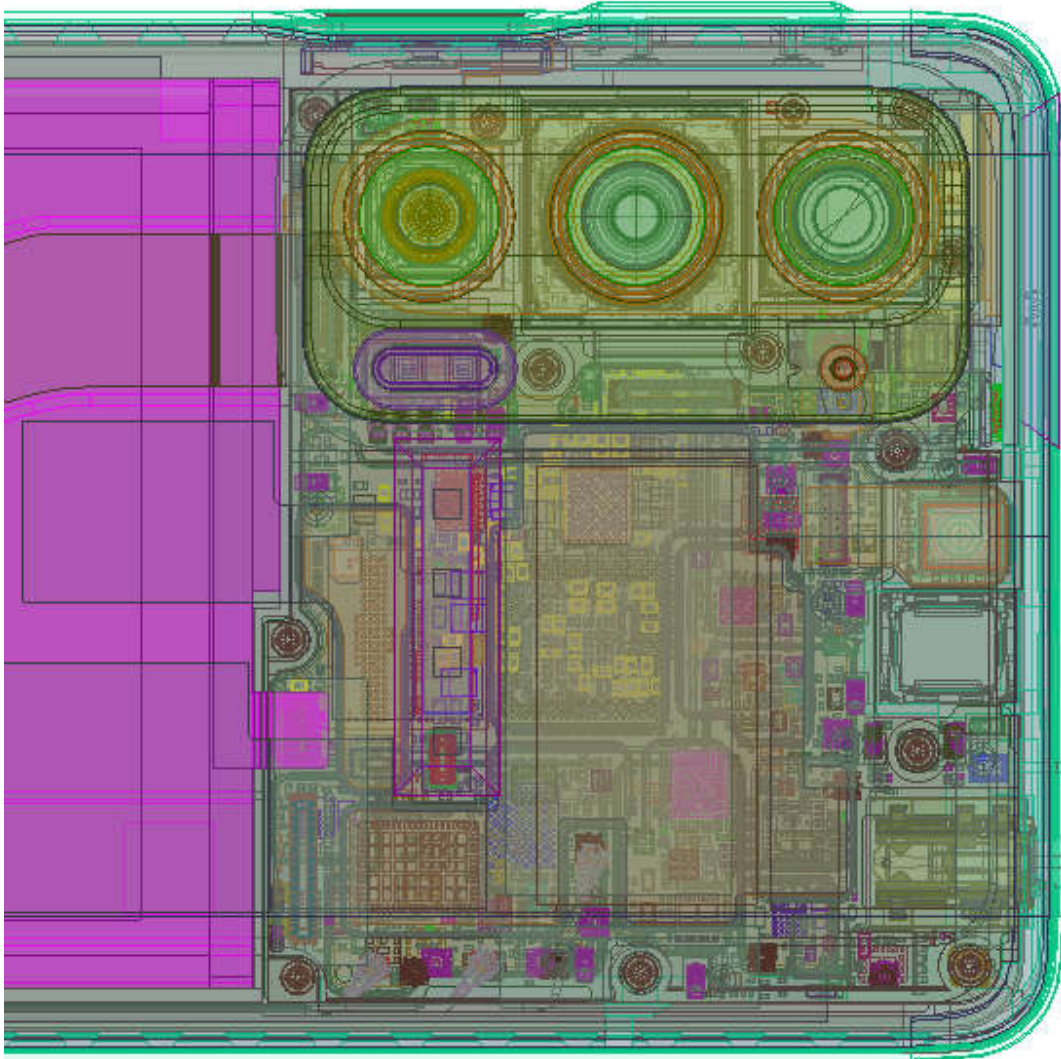
Figure 2.3.4-1: 3D model used for Module 0 (Back module), the antenna array is highlighted
