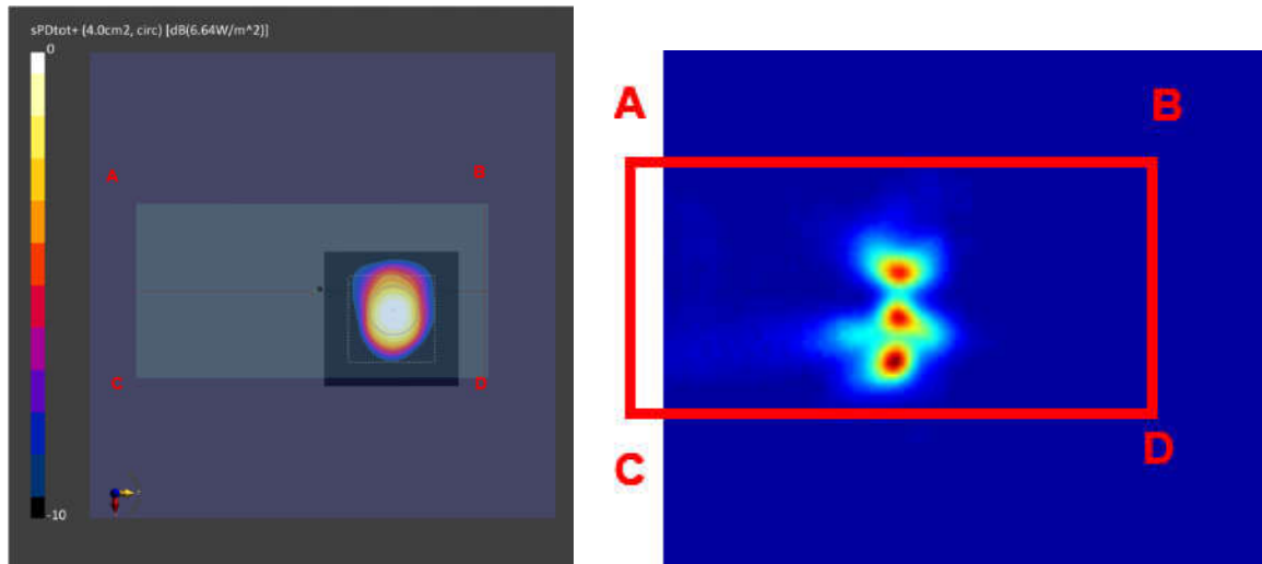
Figure 2.3.7.1-2 Measured (left) and Simulated (right) peak power density distributions for the worst case found in the back surface measurement plane for n261 ( Back module, beam 147, back surface )
