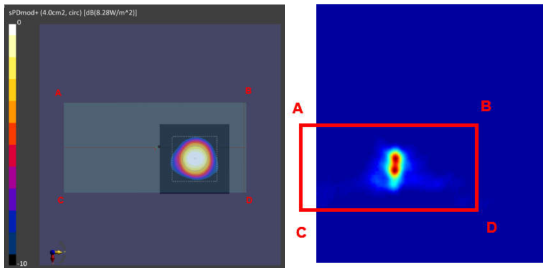
Figure 2.3.7.1-1 Measured (left) and Simulated (right) peak power density distributions for the worst case found in the back surface measurement plane for n261 ( Back module, beam 27, back surface )
