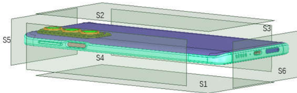
Figure 2.2-1 Identification of the six measurement planes.
