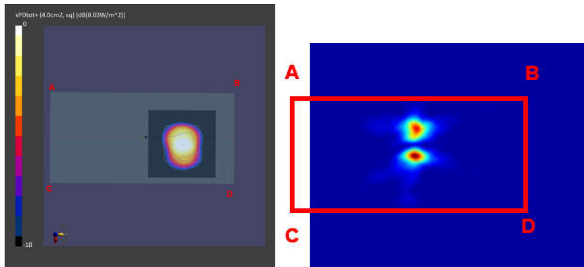
Figure 2.3.7.1-7 Measured (left) and Simulated (right) peak power density distributions for the worst case found in the back surface measurement plane for n260 ( Back module, beam 20, back surface )
