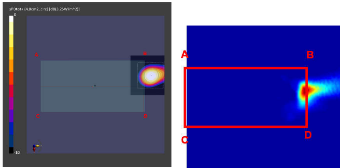
Figure 2.3.7.1-3 Measured (left) and Simulated (right) peak power density distributions for the worst case found in the Top surface measurement plane for n261 ( Top module, beam 23, back surface )
