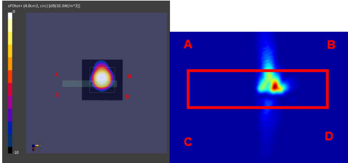
Figure 2.3.7.1-11 Measured (left) and Simulated (right) peak power density distributions for the worst case found in the Top surface measurement plane for n261 (Top module, beam 154, top surface)
