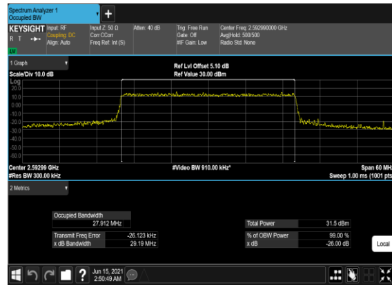
N41(30M)_CP-OFDM_16 QAM_Outer_Full_Mid_CH
