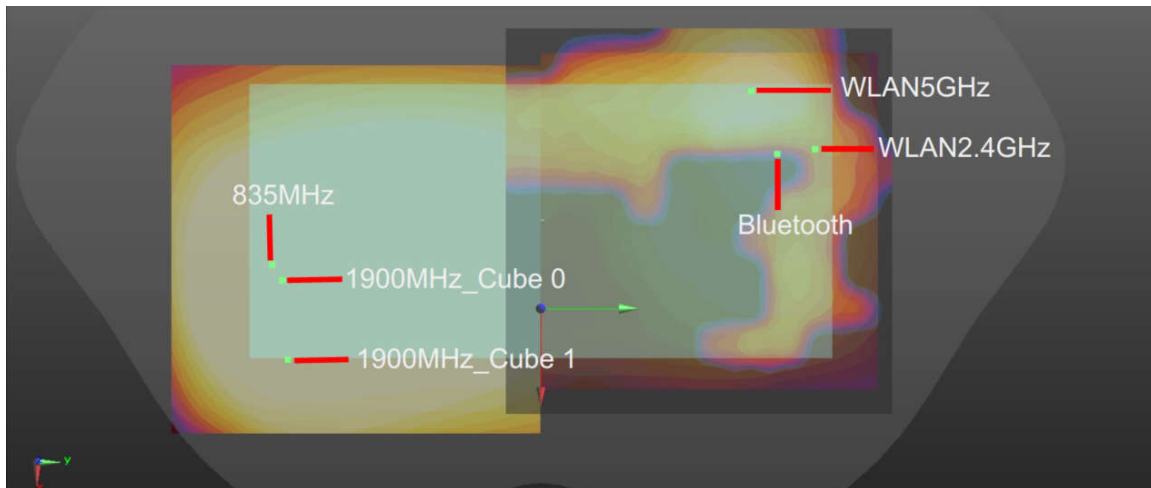
WWAN+2.4GHz/WWAN+WLAN5GHz+Bluetooth_Back_5mm
