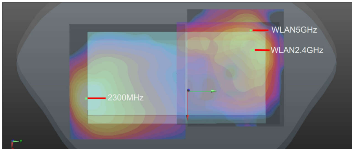
WWAN+2.4GHz/WWAN+WLAN5GHz_Back_0mm
