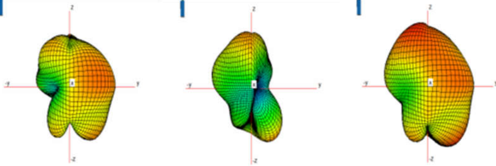
ANT3-WIFI 5G CH1 5500MHz
