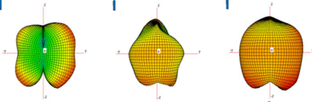
ANT3-WIFI 5G CH1 5800MHz
