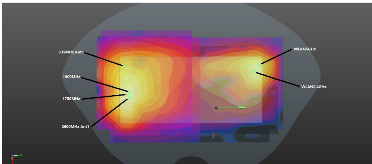
WWAN+WLAN+BT (0mm) Back
