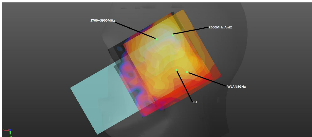
WWAN(ENDC)+WLAN+BT (0mm) Right Check
