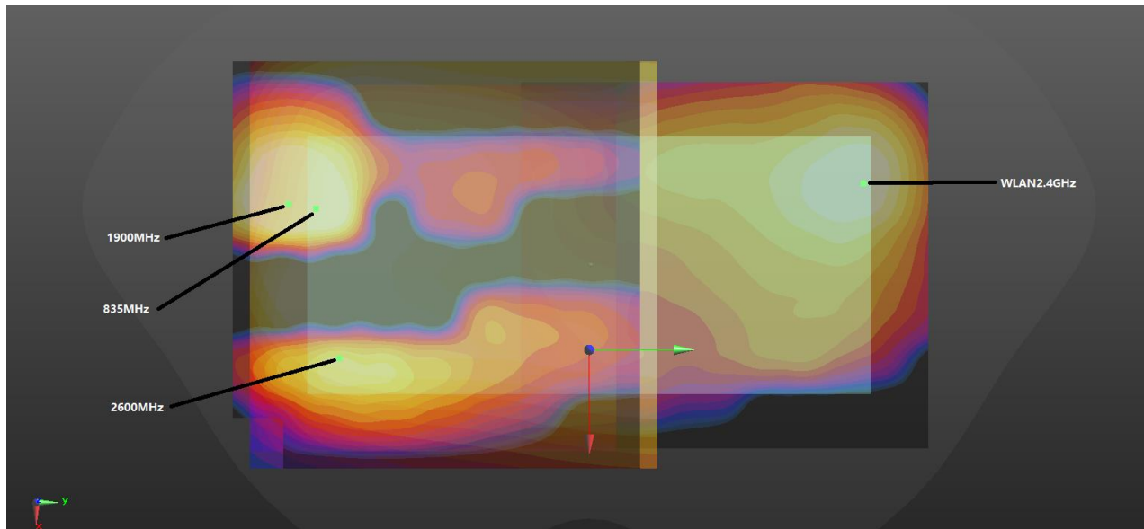
WWAN+WLAN2.4GHz_Back 5mm
