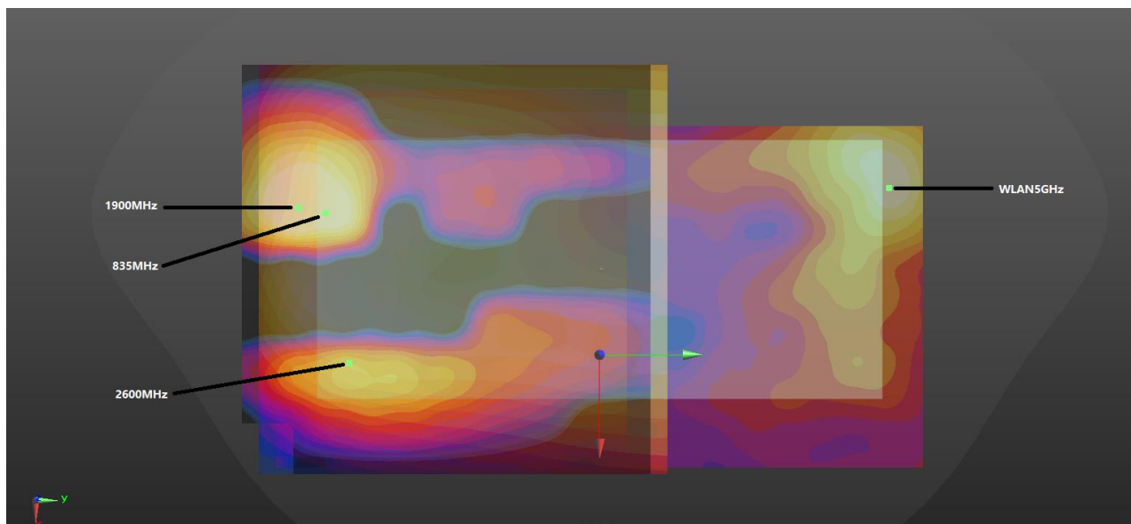
WWAN+WLAN5GHz+Bluetooth_Back 5mm
