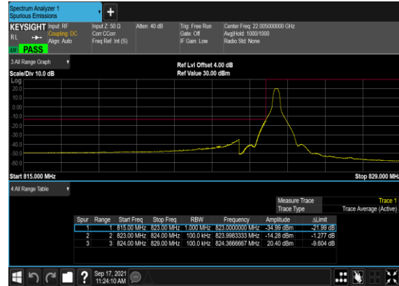
B7_N5(10M)_DFT-s- OFDM_BPSK_Edge_1RB_Left_Low_CH
