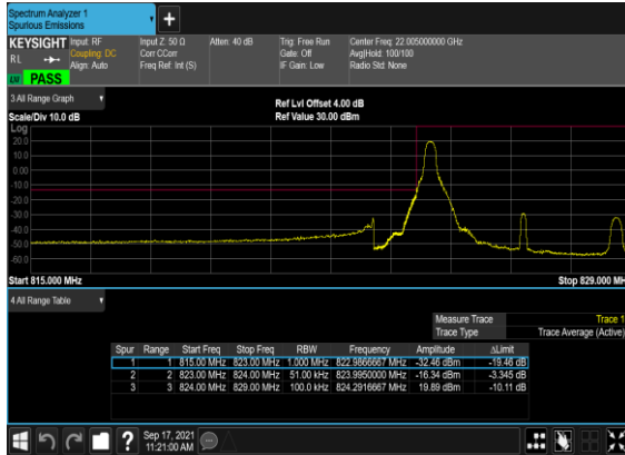
B7_N5(5M)_DFT-s- OFDM_QPSK_Edge_1RB_Left_Low_CH
