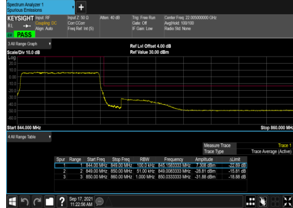
B7_N5(5M)_DFT-s- OFDM_BPSK_Outer_Full_High_CH
