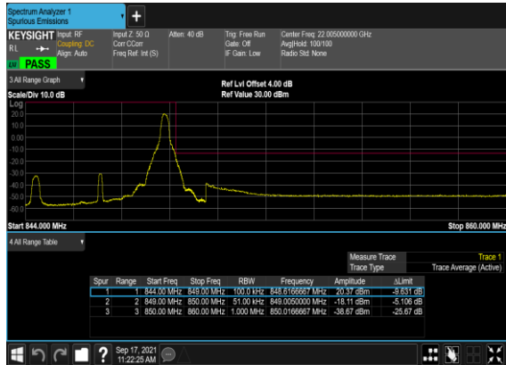
B7_N5(5M)_DFT-s- OFDM_BPSK_Edge_1RB_Right_High_CH
