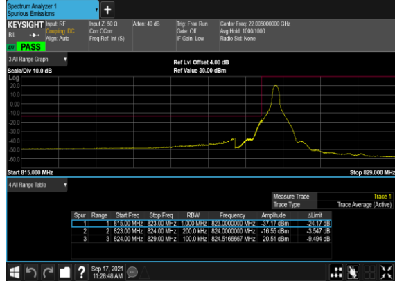
B7_N5(20M)_DFT-s- OFDM_BPSK_Edge_1RB_Left_Low_CH
