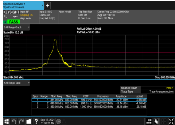
B7_N5(20M)_DFT-s- OFDM_BPSK_Edge_1RB_Right_High_CH
