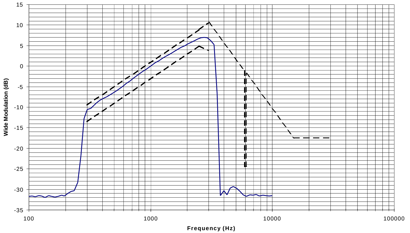
Tx Audio Response -- Wide Mode
