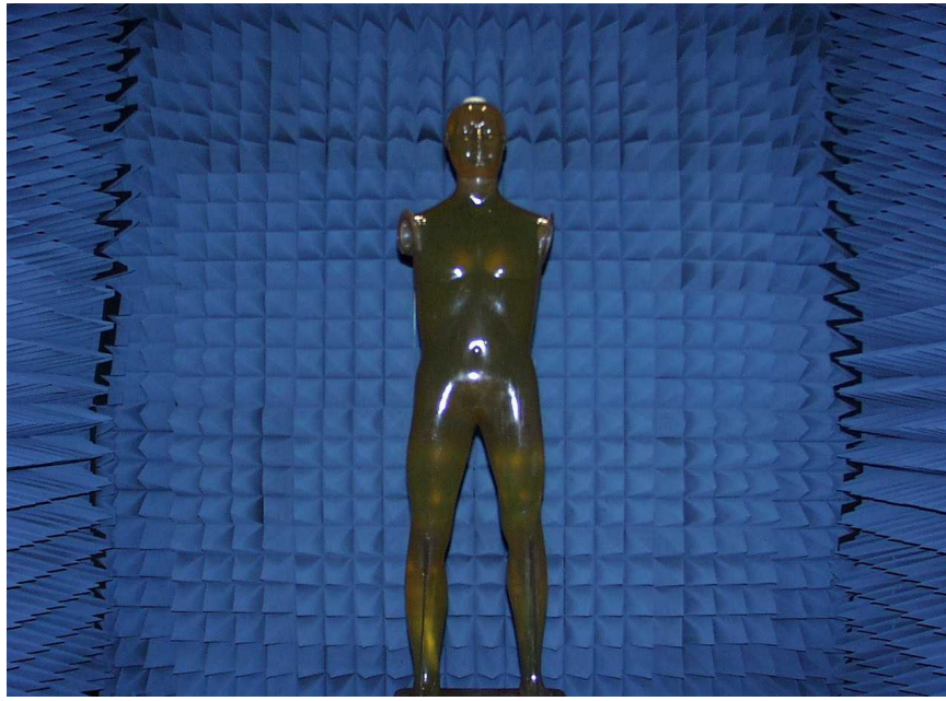
Figure 7. Phantom in Anechoic Chamber.
