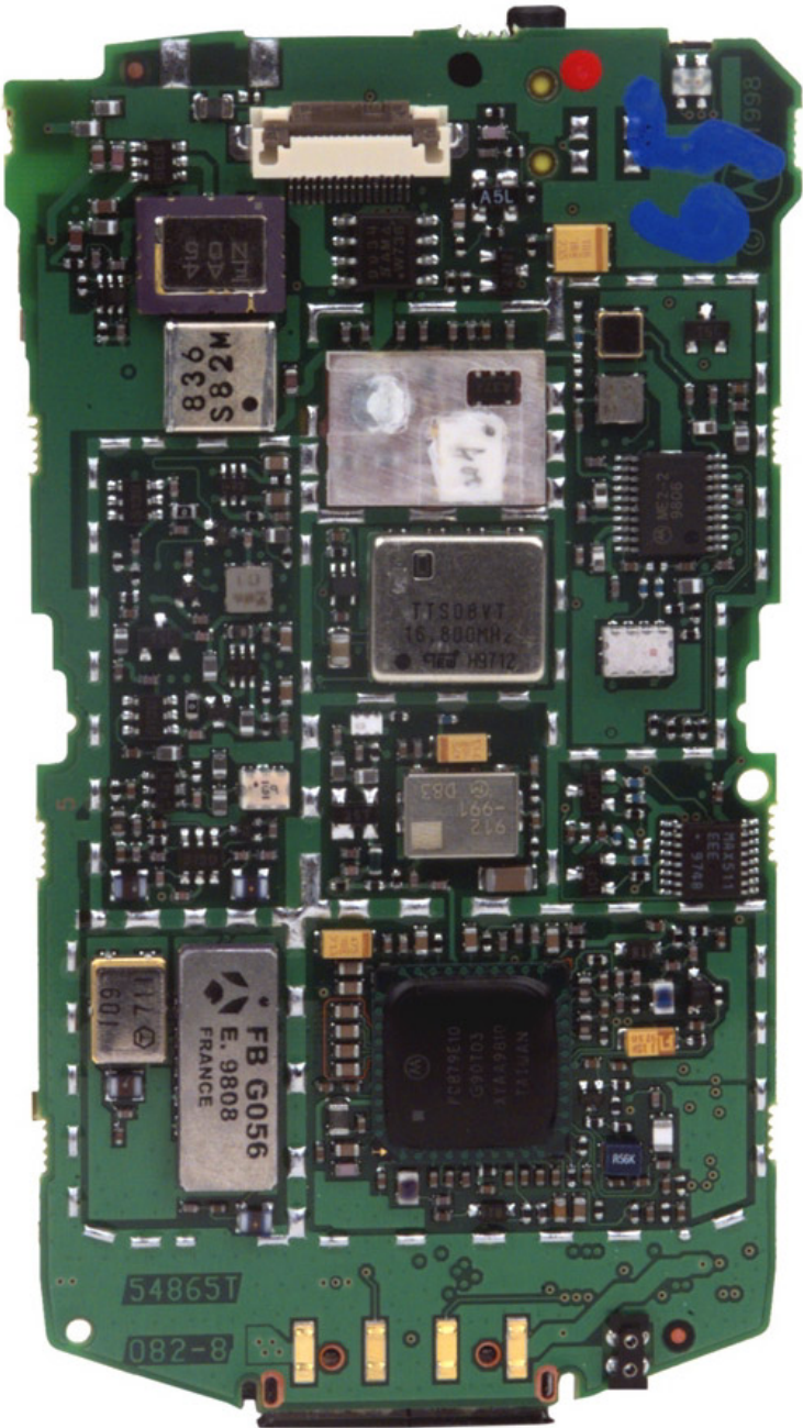
Transceiver Board
