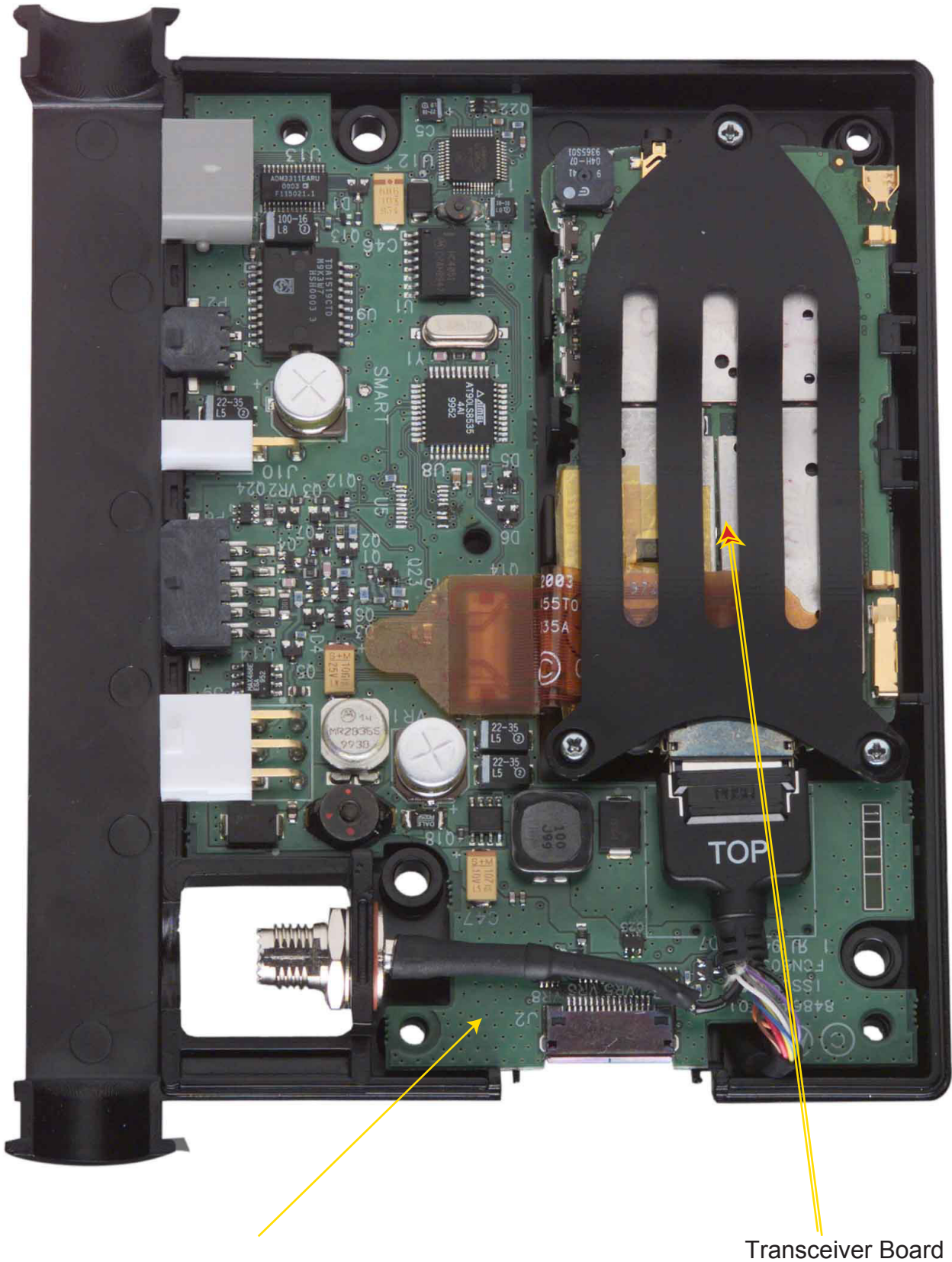
Interface Board
