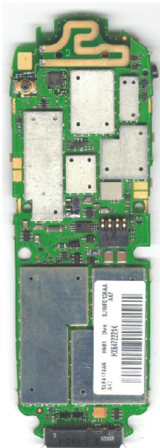
Rear View
