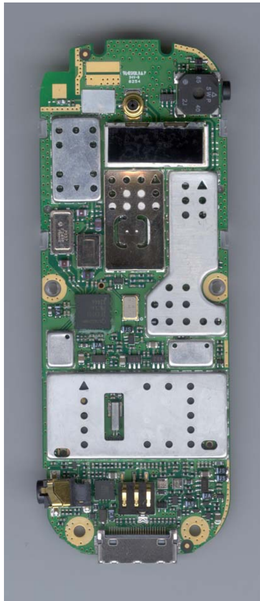
Rear View
