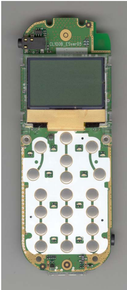
Front View
