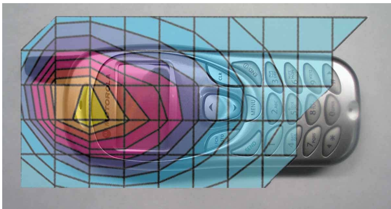
Figure 4. Typical 800MHz Right Head Adjacent Contour Overlaid on Phone with Antenna Fixed (15 ° Tilt)
