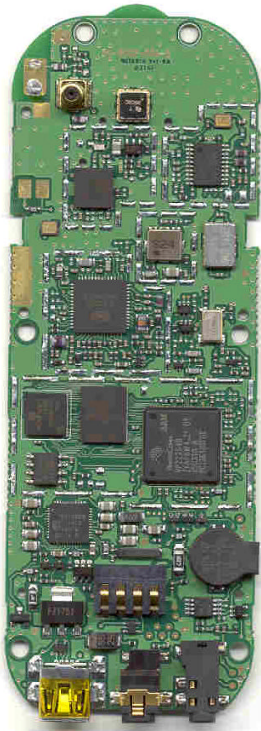
Rear View (Shields Removed)
