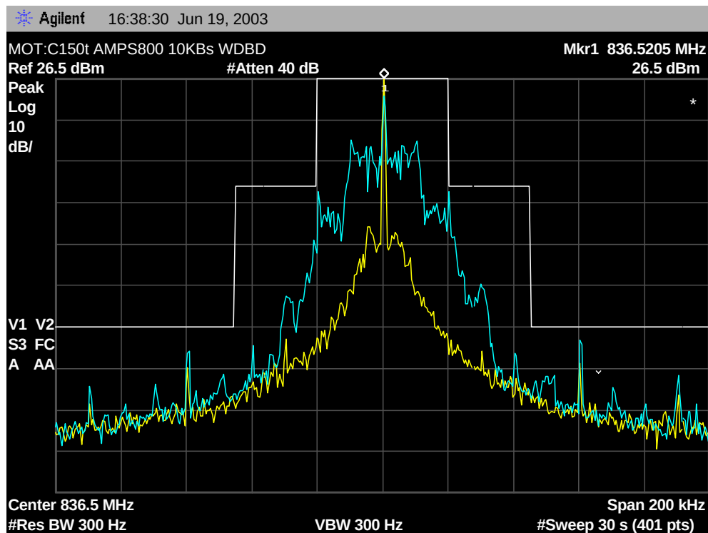
AMPS 800 10KBs Wideband
