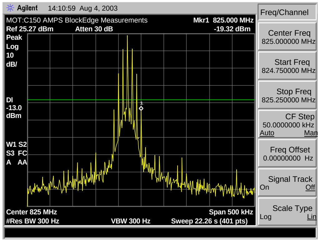
Block A* (Lower) Max Edge
