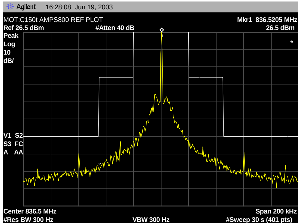
AMPS 800 Reference Plot
