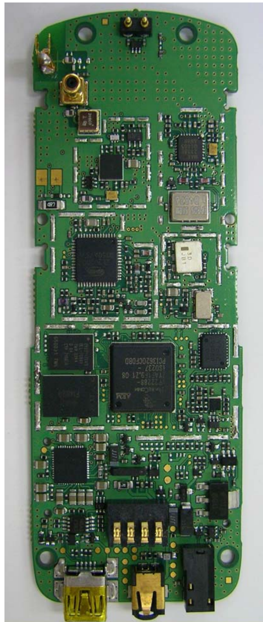
REAR VIEW WITHOUT SHIELDS
