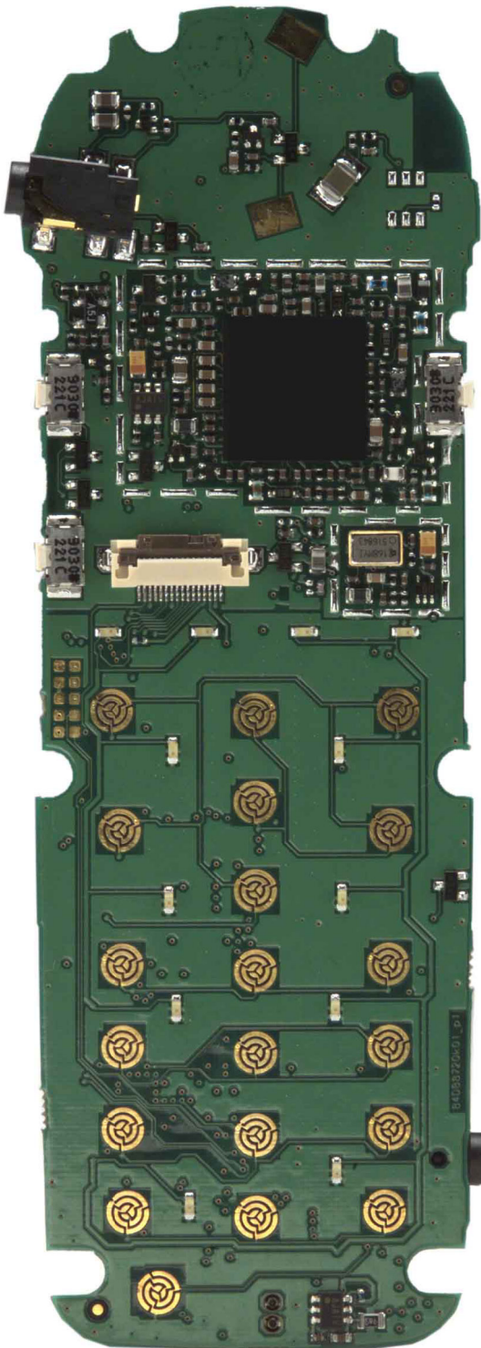
Front View (Shields Removed)
