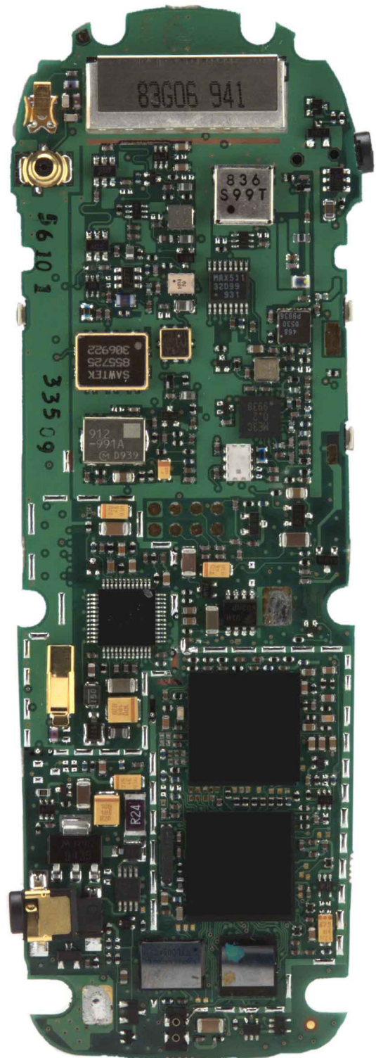
Rear View (Shields Removed)
