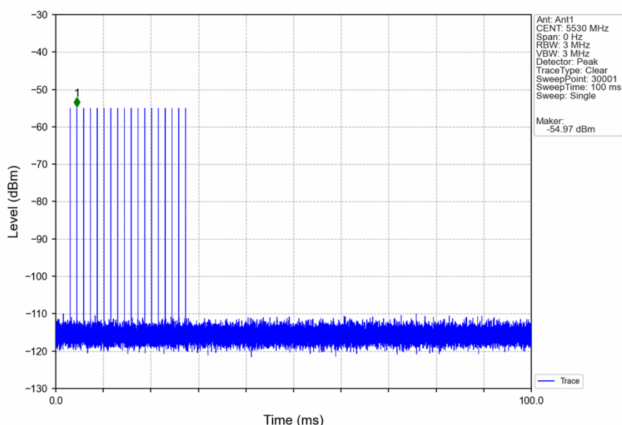
Signal Calibration_802.11ac(VHT80)_2C_5530MHz_RadarType1_Trial0
