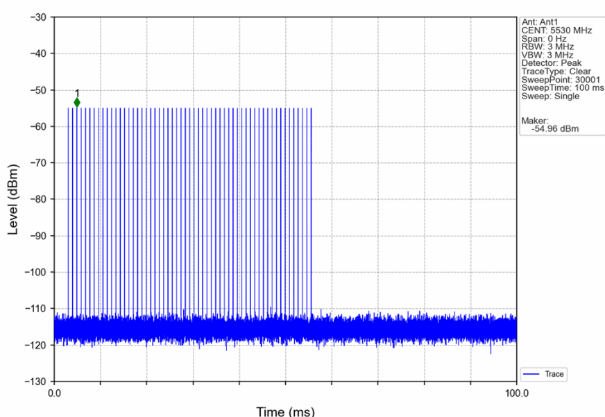
Signal Calibration_802.11ac(VHT80)_2C_5530MHz_RadarType1_Trial0
