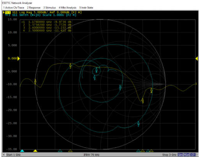
BT Gain:-8.69dBi (PEAK)
