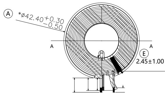
Coil Antenna
