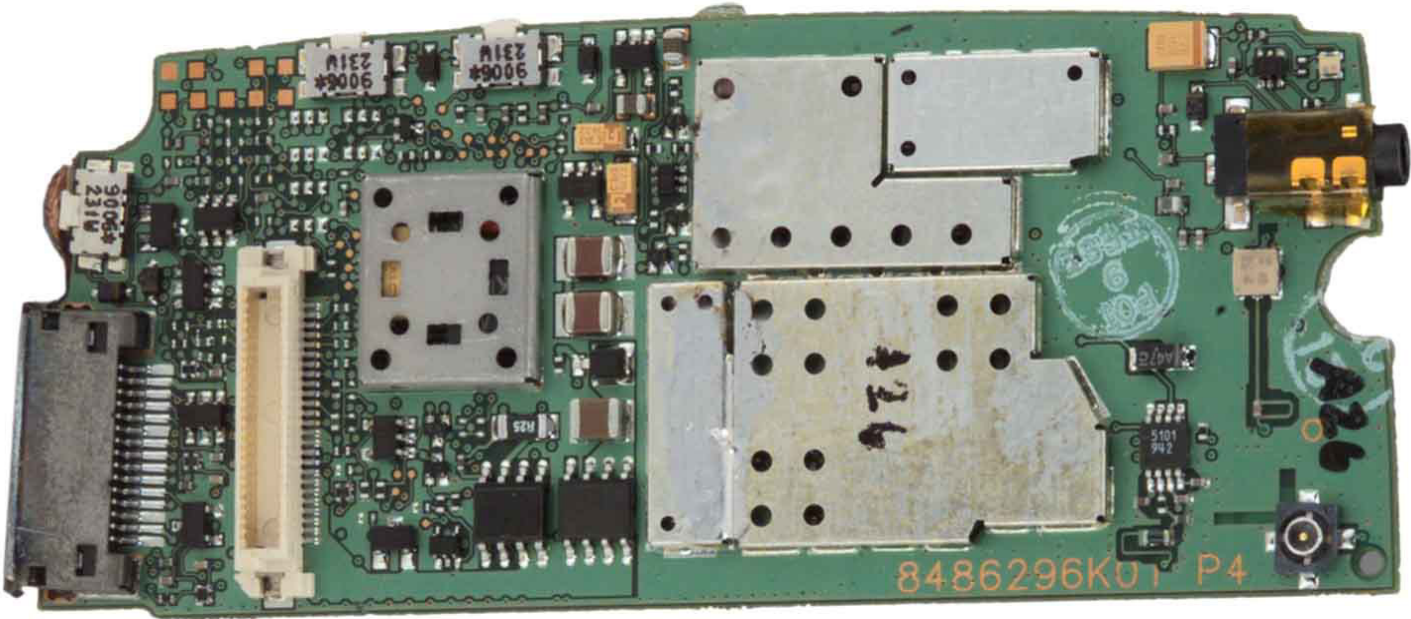
RF Board Side 1
