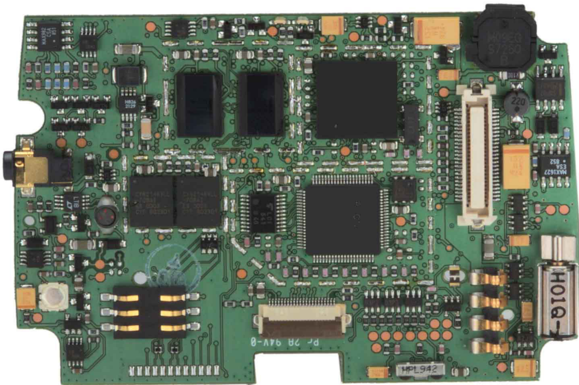
Logic Board Rear View
