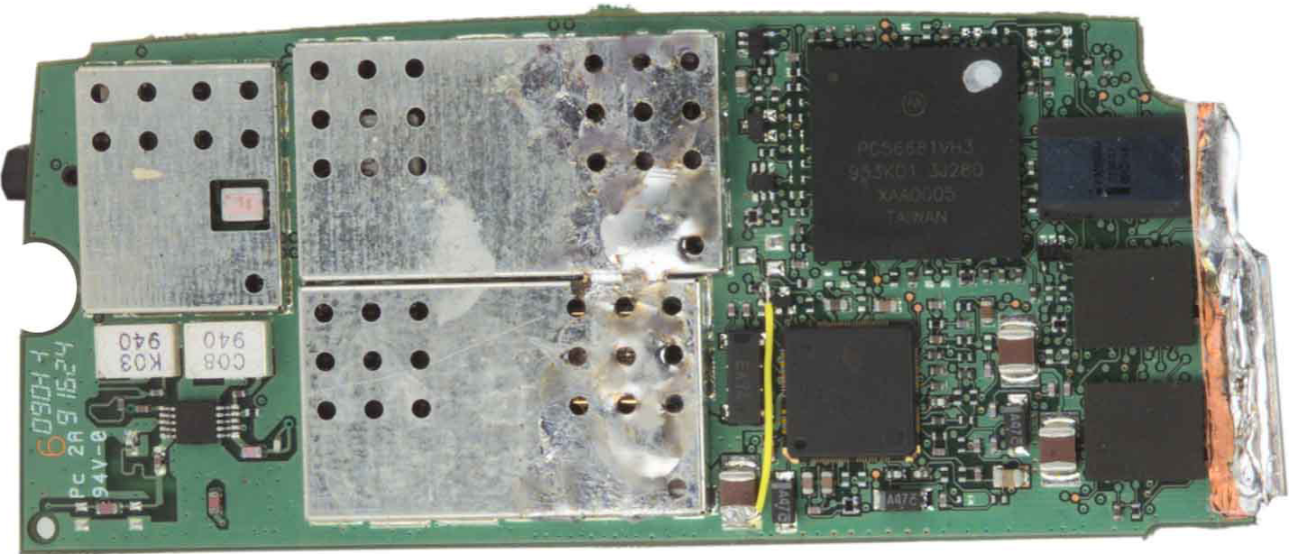
RF Board Side 2
