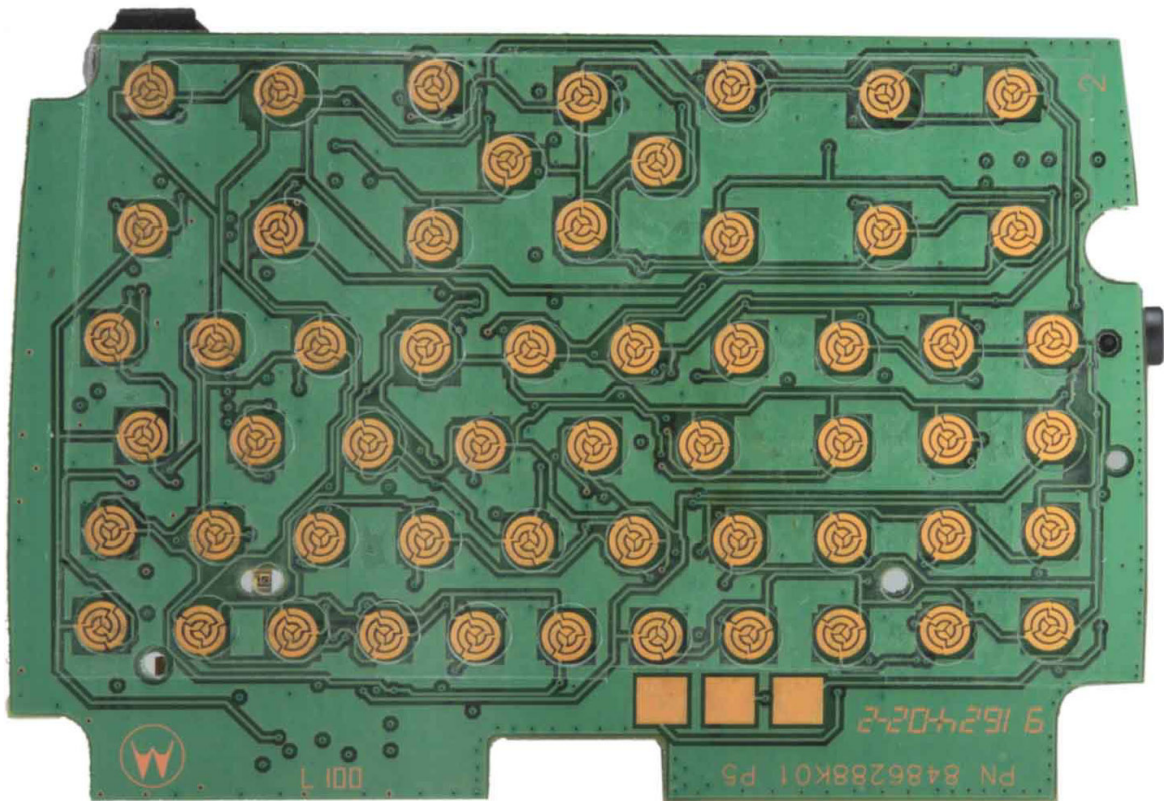
Logic Board Front View
