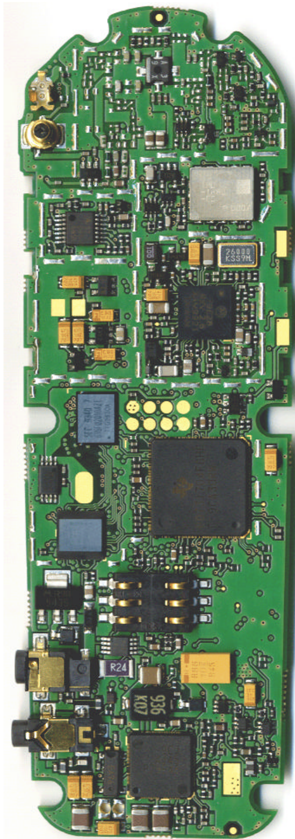
BOTTOM VIEW (SHIELDS REMOVED)
