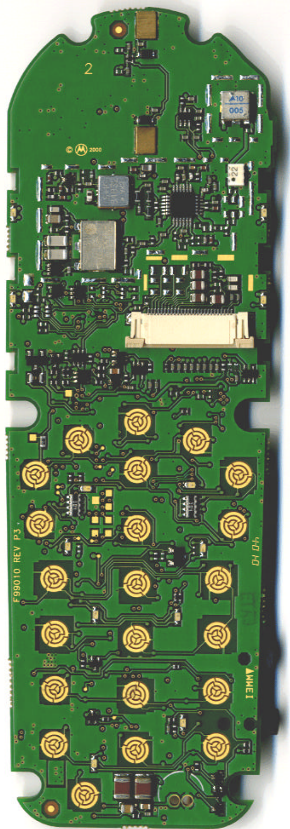
TOP VIEW (SHIELDS REMOVED)
