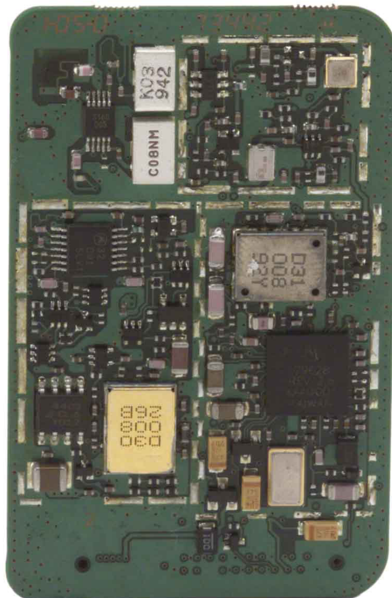
RF Board Side 2 (Shields Removed)
